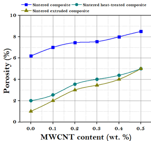
Figure 7: Porosity of the composites with varying weight percentages of MWCNTs.
