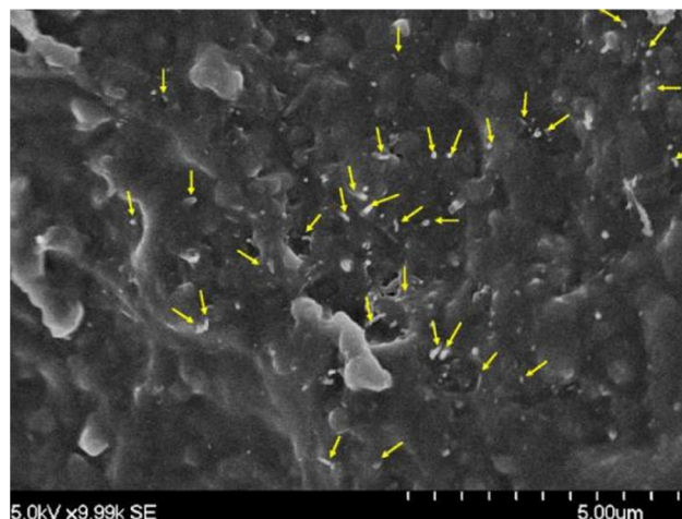
Figure 17: The SEM image shows that the MWCNTs in the sample containing 1.5 wt% COOH-MWCNTs are distributed in the epoxy resin matrix [90].
