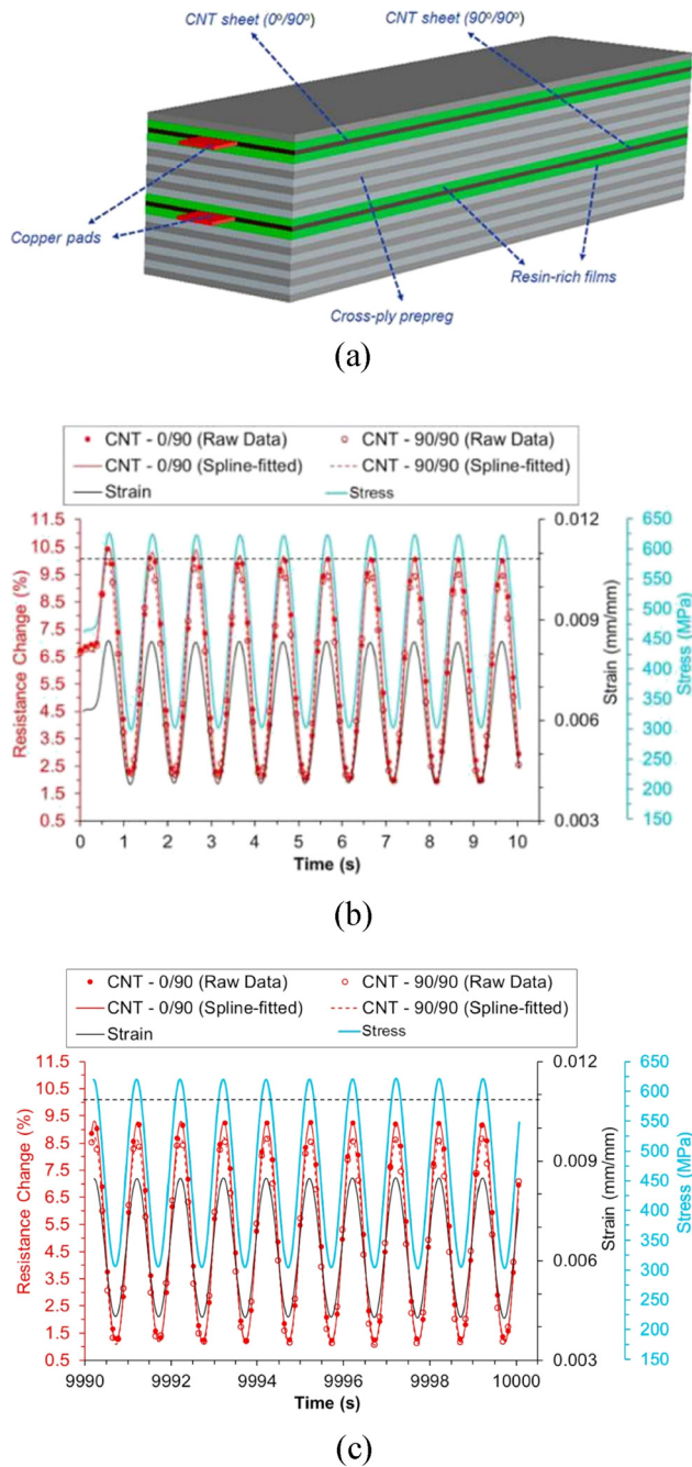
Figure 25: (a) Lay-up sequence of the CNT sheet integrated in a cross-ply carbon-epoxy laminate for fatigue test; (b) and (c) real-time electrical and mechanical response under cyclic fatigue loading of the carbon fiber laminates with integrated CNT sheets during first ten cycles and last ten cycles of the fatigue testing (dashed line showing the initial peak magnitude of the electrical resistance) [157].
