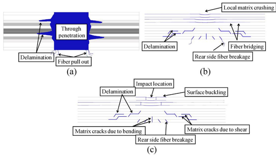
Figure 18: Schematic showing different damage mechanisms due to impact load: (a) high energy, (b) medium energy, and (c) low energy [97].
