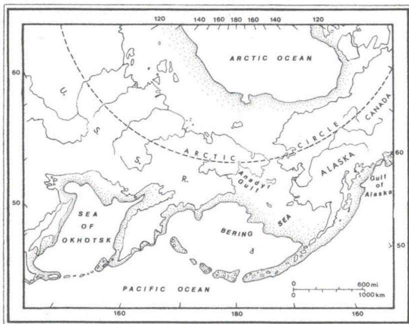
Beringia at Würm maximum. (Derived from Hopkins 1972; Haag 1962).
