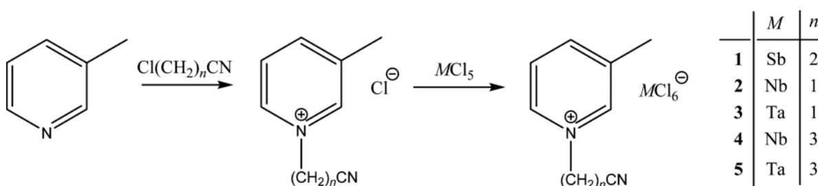
Scheme 1. Synthesis of the nitrile-functionalized pyridinium chlorides and hexachloridometalate(V) salts 1–5 .
