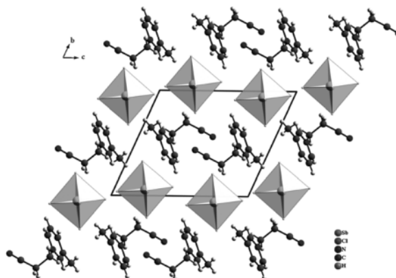
Fig. 1. Projection of the crystal structure of [(CH_2)_2CNmpy][SbCl_6] ( 1 ) along the crystallographic a axis.
