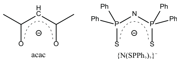
Fig. 1. The ligands acac vs. \{N(SPh_2)_2\}^- .
