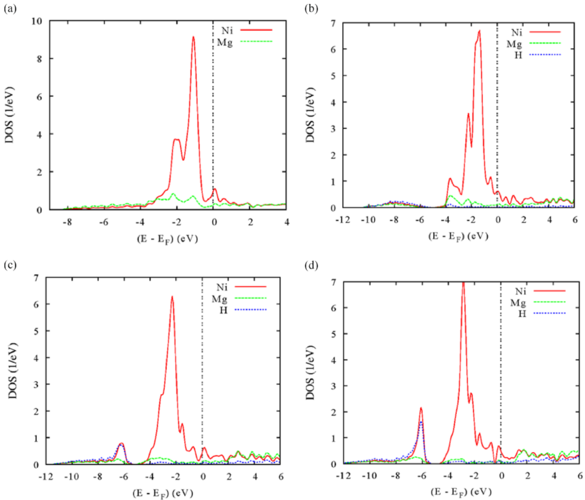
Fig. 2 (color online). Site projected density of states: a) MgNi, b) MgNiH, c) MgNiH 2 , and d) MgNiH 3 .
