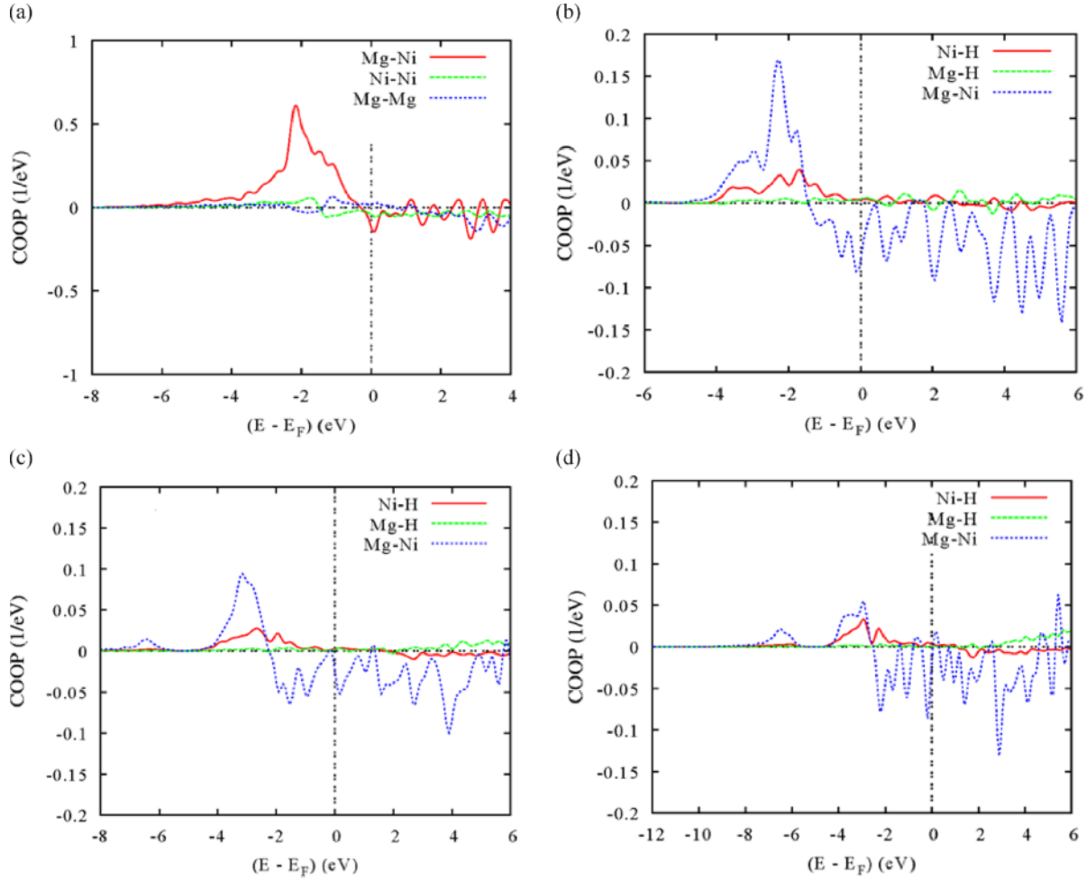
Fig. 3 (color online). Chemical bonding for pair interactions (atom-to-atom) of a) MgNi, b) MgNiH, c) MgNiH 2 , and d) MgNiH 3 .
