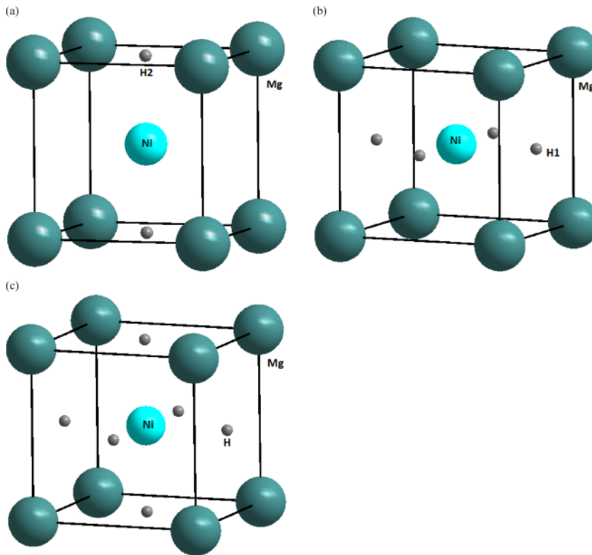
Fig. 1 (color online). \text{MgNiH}_x : the three model structures used in the calculations; a) \text{MgNiH} ; b) \text{MgNiH}_2 ; c) \text{MgNiH}_3 (vertical: tetragonal axis c ).
