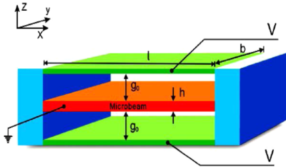
Fig. 1 (colour online). Schematics of a double-sided driven clamped-clamped microbeam-based electromechanical resonator.
