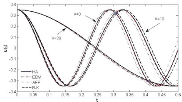
Fig. 3. Comparison between Hamiltonian approach (HA), amplitude–frequency formulation (AFF), energy balance method (EBM), and the fourth-order Runge–Kutta method (R-K); A = 0.35 .
