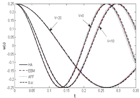
Fig. 2. Comparison between Hamiltonian approach (HA), amplitude–frequency formulation (AFF), energy balance method (EBM), and the fourth-order Runge–Kutta method (R-K); A = 0.25 .
