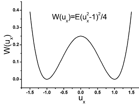
Fig. 1. Double-well potential energy density W(u_x) .
