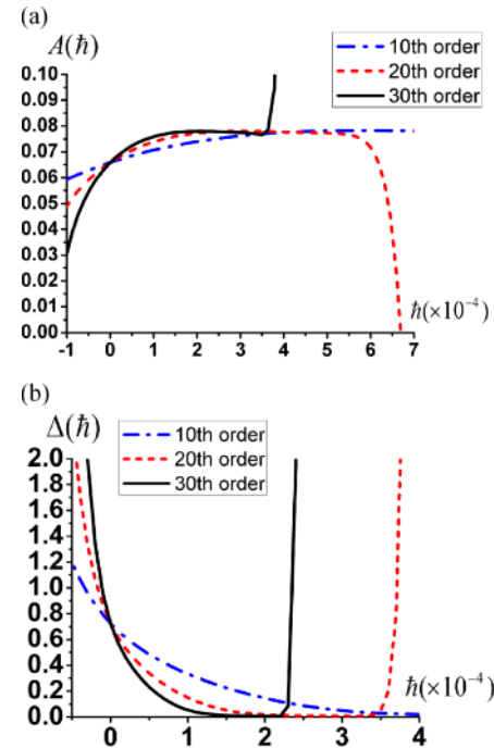
Fig. 2 (colour online). Two criteria to judge convergence ( \bar{\alpha} = 0.00015 , \bar{\beta} = 15 , k = 5 , d = 0 ); (a) A(\hbar) of 10th, 20th, 30th-order of approximation, (b) residual integral \Delta(\hbar) of 10th, 20th, 30th-order of approximation.
