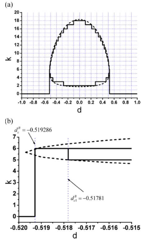
Fig. 5 (colour online). k - d bifurcation diagram of parameter set B: \bar{\alpha} = 0.00015 , \bar{\beta} = 15 ; (a) whole view, (b) local view near bifurcation.
