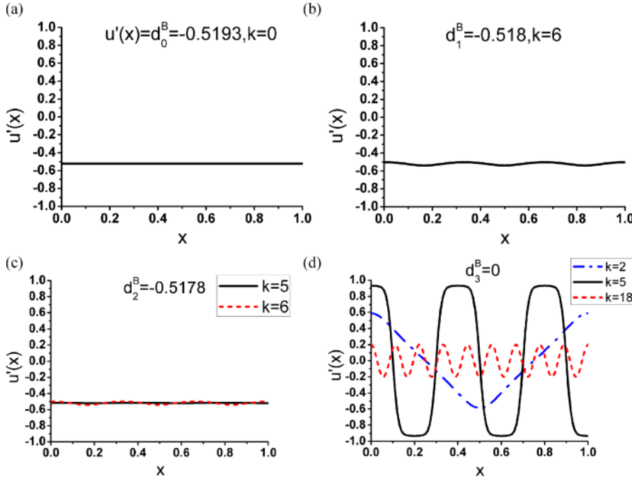
Fig.6 (colour online). Solution(s) for the strain u'(x) at different values of load d of parameter set B: \bar{\alpha} = 0.00015 , \bar{\beta} = 15 . (a) Classical homogeneous solution ( k = 0 ) at d_0^B = -0.5193 < d_{c1}^B = -0.519286 with no phase transition. (b) Only inhomogeneous solution ( k = 6 ) at d_1^B = -0.518 < d_{c1}^B = -0.51781 . (c) Emergence of the double solutions ( k = 5, 6 ) at d_2^B = -0.5178 > d_{c1}^B = -0.51781 . (d) Three of the many solutions ( k = 2 \sim 18 ) at d_3^B = 0 .
