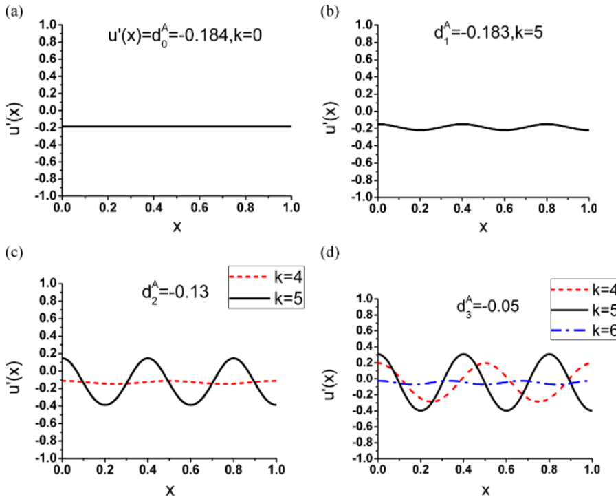
Fig. 4 (colour online). Solution(s) for the strain u'(x) at different values of load d of parameter set A: \bar{\alpha} = 0.001 , \bar{\beta} = 50 . (a) Classical homogeneous solution ( k = 0 ) at d_0^A = -0.184 < d_c^A = -0.183698 with no phase transition. (b) Emergence of the only inhomogeneous solution ( k = 5 ) at d_1^A = -0.183 > d_c^A , hence the martensitic transformation occurs. (c) Emergence of the double inhomogeneous solutions ( k = 4, 5 ) at d_2^A = -0.13 > d_{c1}^A = -0.13028 . (d) Emergence of the triple inhomogeneous solutions ( k = 4, 5, 6 ) at d_3^A = -0.05 > d_{c2}^A = -0.05145 .
