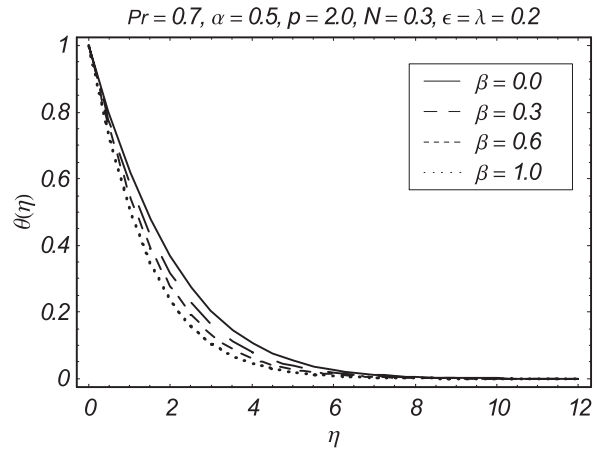
Fig. 8. Influence of \beta on \theta(\eta) .
