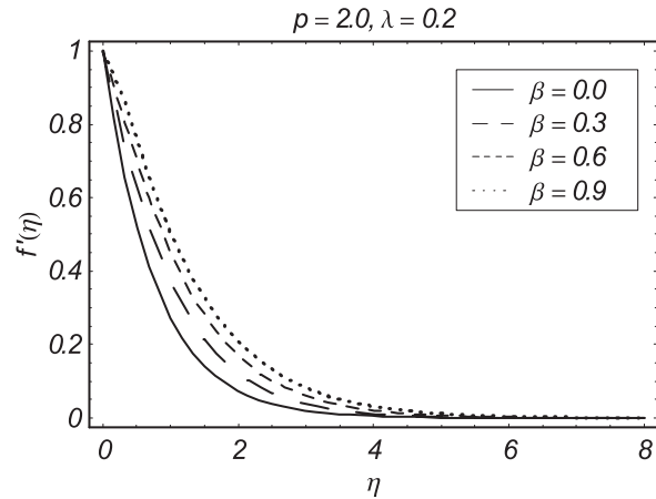
Fig. 2. Influence of \beta on f'(\eta) .
