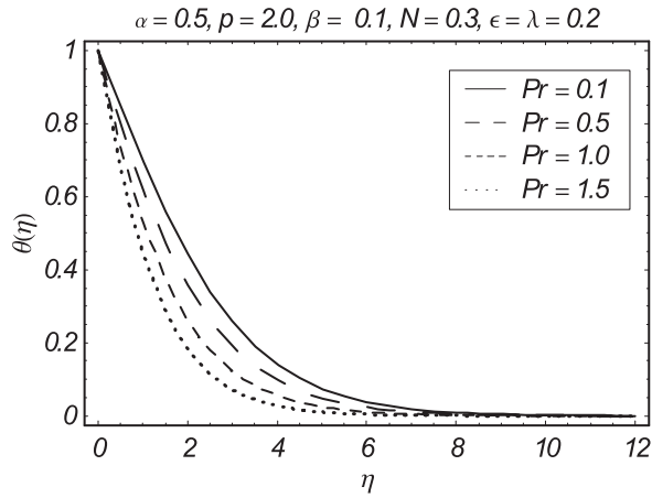
Fig. 5. Influence of Pr on \theta(\eta) .
