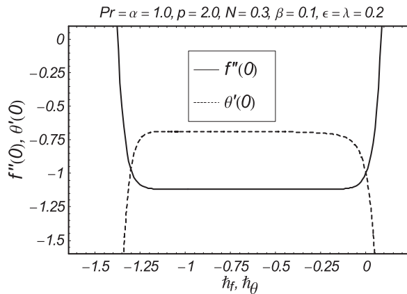
Fig. 1. h -curves for the functions f and \theta .
