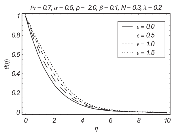
Fig. 10. Influence of \epsilon on \theta(\eta) .
