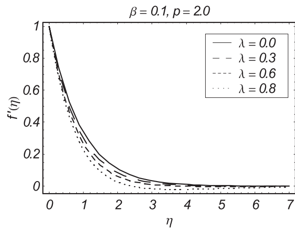
Fig. 4. Influence of \lambda on f'(\eta) .
