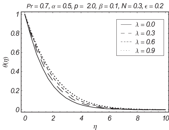
Fig. 11. Influence of \lambda on \theta(\eta) .
