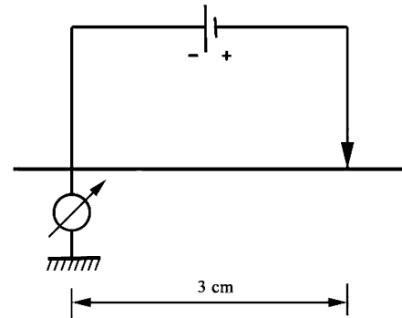
Fig. 7. Circuit diagram used for the detection of transient currents.
