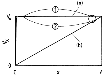
Fig. 2. Potential distribution (a) along the high-conducting current path and (b) along the adjacent low-conducting matrix, with a current flowing through the sample between cathode C and anode A and the potential probes placed as indicated, when the voltage V_h is very small.
