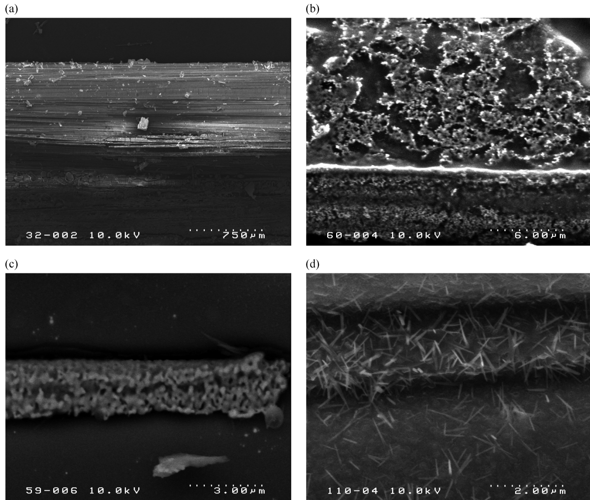
Fig. 6. SEM images (recorded at 10 kV) of a high-conducting sample area, taken in the secondary electron-mode with increasing magnification. (a) High-conducting path of 600 \mu\text{m} width. (b) Two high-conducting filaments visible below the white track. (c) Detailed view of one high-conducting filament. (d) Three closely packed high-conducting filaments.
