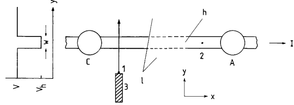
Fig. 4. Potential differences V and V_h of a mobile potential probe against a fixed potential probe at locations y perpendicular to the current path, when in the x -direction a current I flows through the sample. The notation is 1, mobile potential probe; 2, fixed potential probe; 3, micrometer head; C, cathode; A, anode; h , high-conducting current path; l , low-conducting matrix; and w , width of high-conducting current path.
