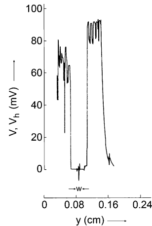
Fig. 5. Potential differences V and V_h of a mobile potential probe against a fixed potential probe. The mobile potential probe is moved from some origin y = 0 , positioned on the low-conducting matrix below the high-conducting current path, towards the upper boundary of the sample, passing with increasing y across the high-conducting current path of width w . The distance between the two potential probes in the direction of current flow is 2 cm; the current I flowing through the sample is 1 A.
