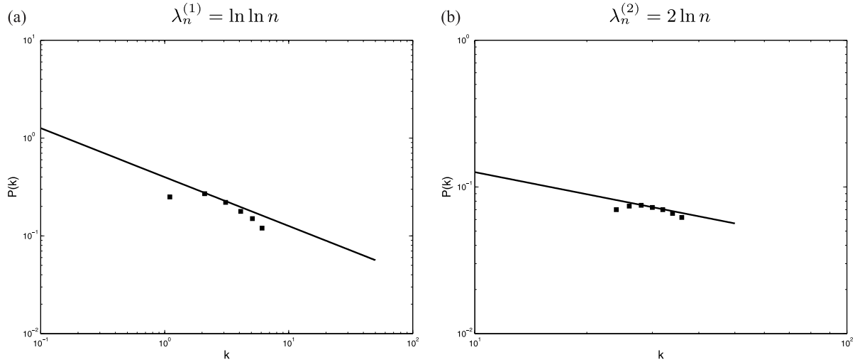
Fig. 1. Connectivity degree P(k) for classical random graph G(n, \lambda_n^{(i)}/n) for i = 1, 2 with n = 10^5 . The solid curves represent the analytical curve 1/\sqrt{2\pi k} , and the squares are for simulation results.
