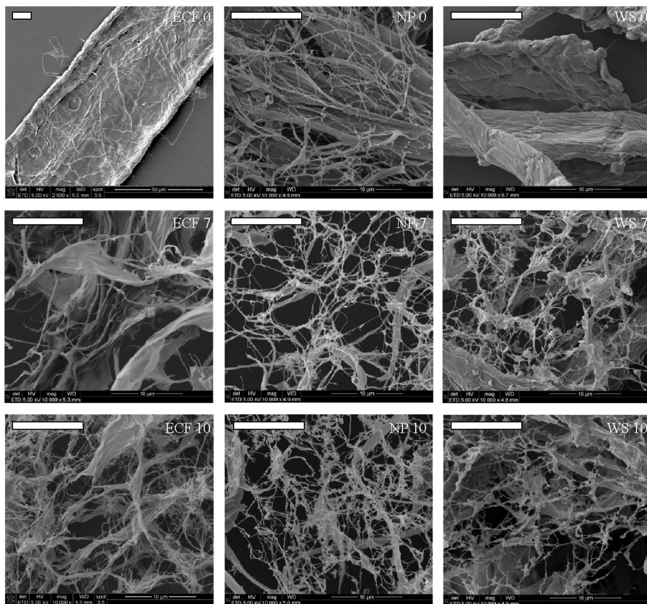
Fig 2 - SEM micrographs of the different materials after 0, 7 and 10 grinding cycles. Scale bar is 10 \mu m.
