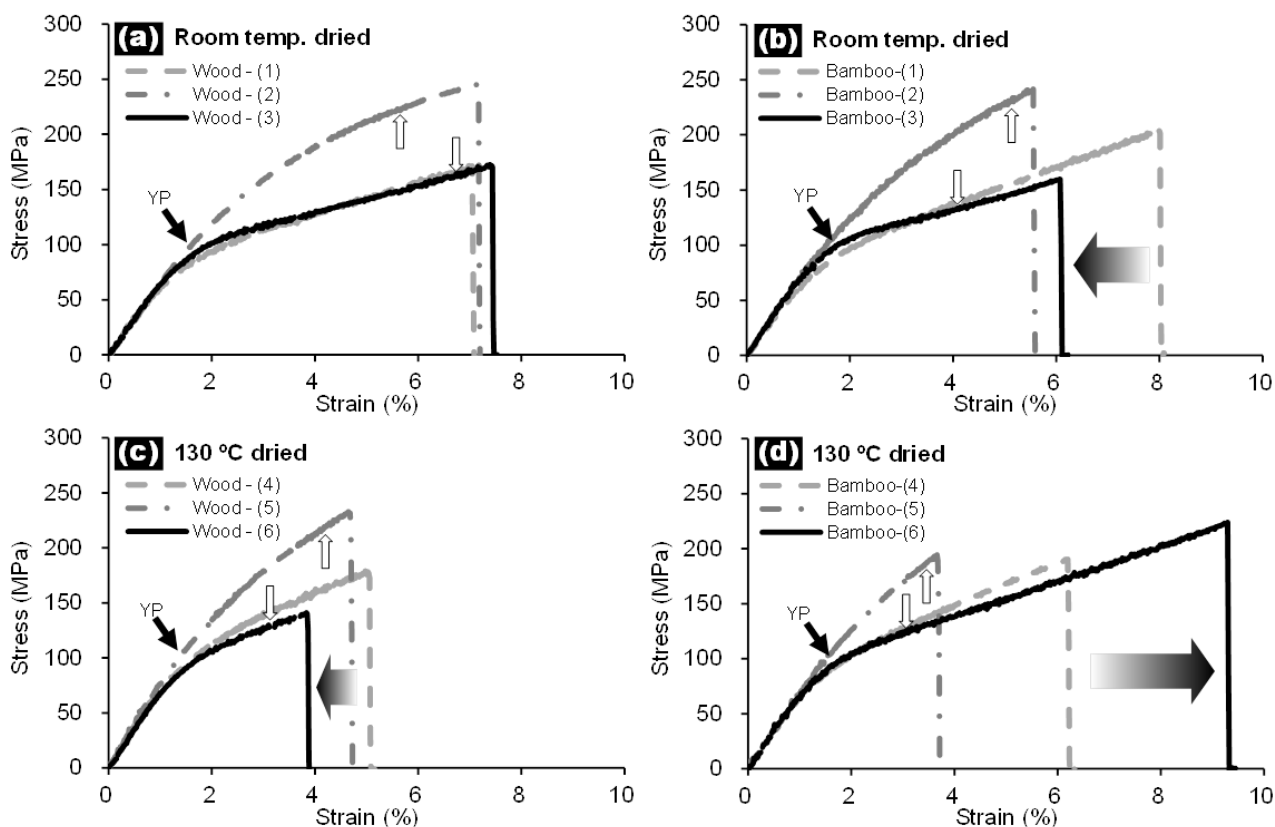
Fig 6 - Tensile stress-strain curve of room temperature-dried CNF sheets derived from wood (a) and bamboo (b), and of 130 °C dried CNF sheets derived from wood (c) and bamboo (d). Measurement conditions of the sheets (1)-(6) were indicated in Fig 4. The close arrows (YP) indicate the yield points. The larger arrows indicate changing of strain-to-failure followed by desorption and subsequent absorption of water. The open arrows indicate change of stress-strain curve by changing humidity-condition. The slash areas indicate elastic regions.
