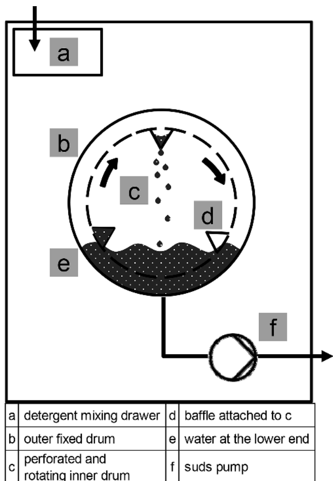
Figure 1 Standard-System with passive baffles
