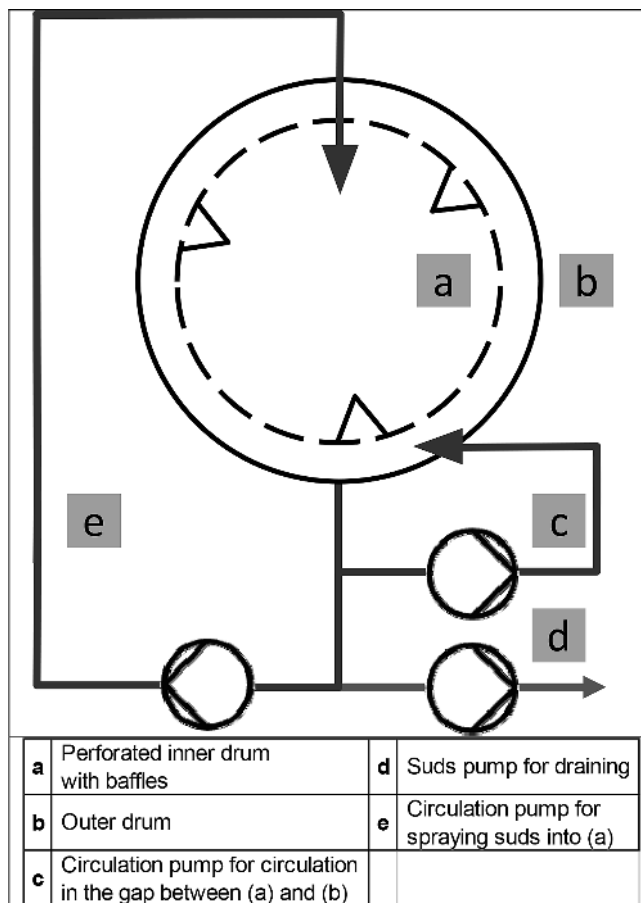
Figure 2 Illustration of different waterways
