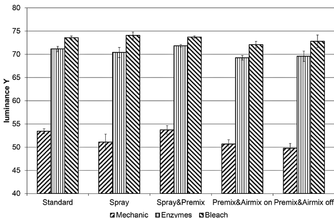
Figure 4 Mean luminance of stain groups as measure of washing performance
