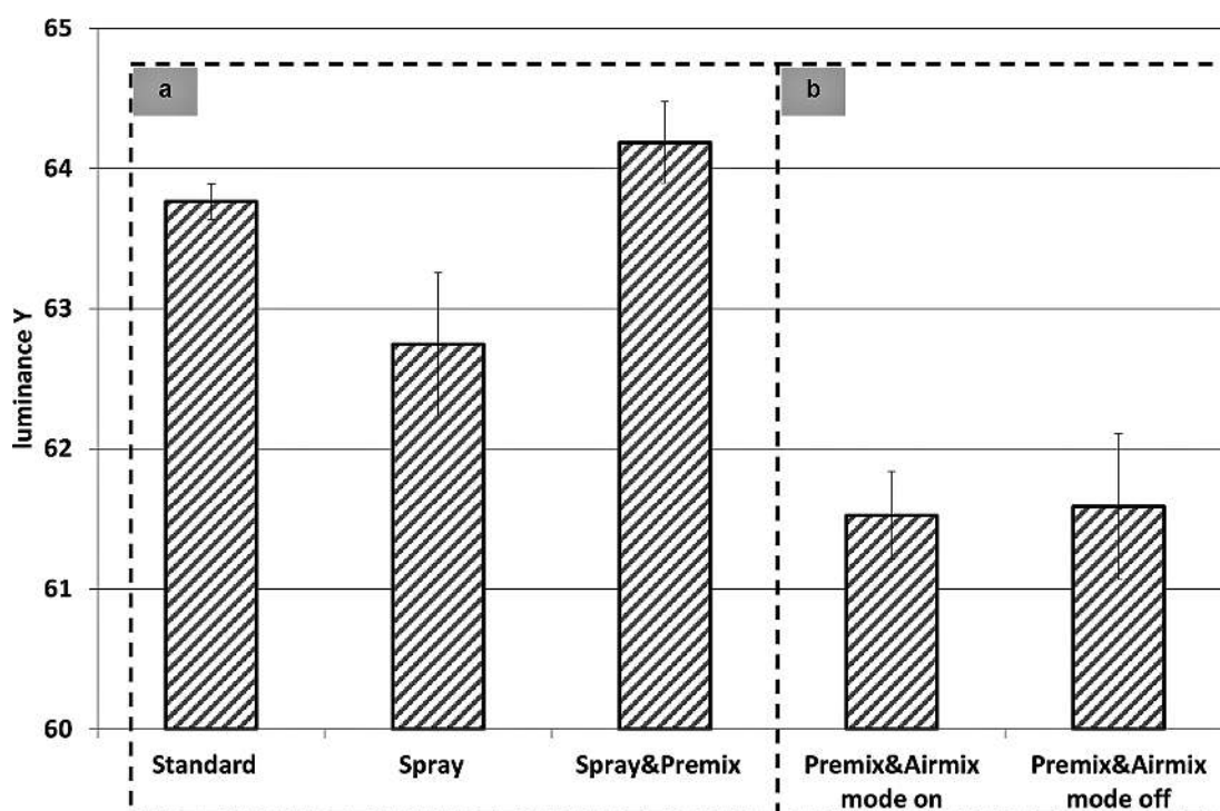
Figure 3 Mean luminance as relative measure of washing performance. a: Systems with long main wash time; and b: Systems with short main wash time. Error bars show confidence intervals at 95%-level
