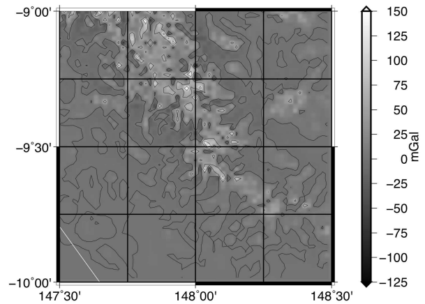
Figure 6. Downward continuation effect of Jacobi method using a tolerance of 6.7 mGal.
