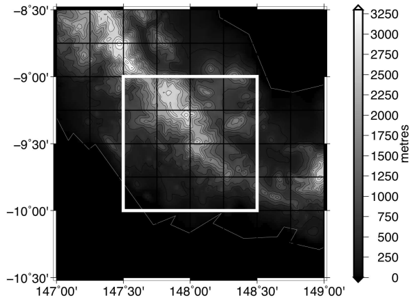
Figure 2. Heights of topography over the study area.
