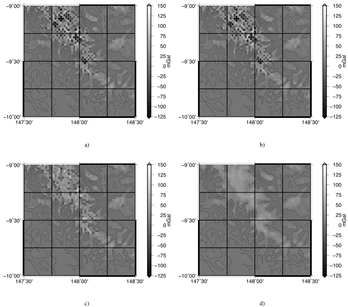
Figure 4. Downward continuation effect from the Jacobi iterative method with testing of the \delta^t vector with a) 0.05 mGal, b) 0.5 mGal, c) 5 mGal and d) 50 mGal tolerances.
