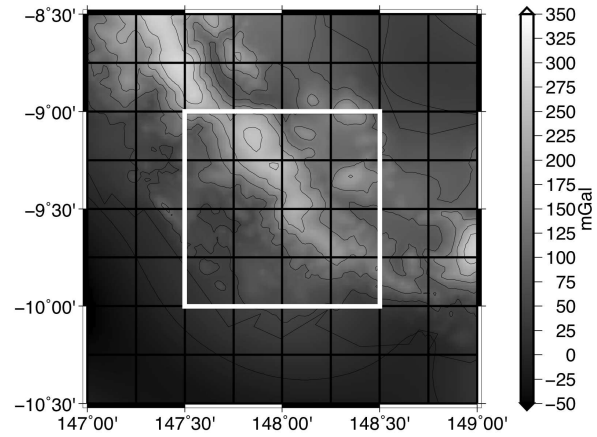
Figure 1. Helmert gravity anomalies over the study area.
