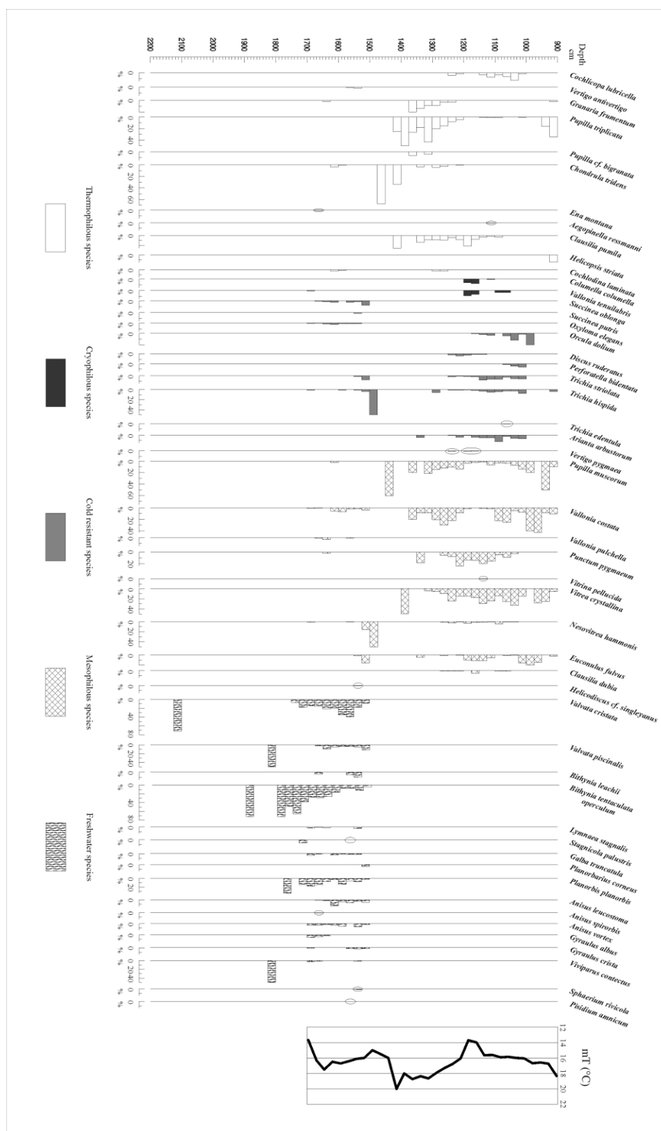
Figure 4. The dominance relationships of the mollusc species from the profile with malacothermometer data.
