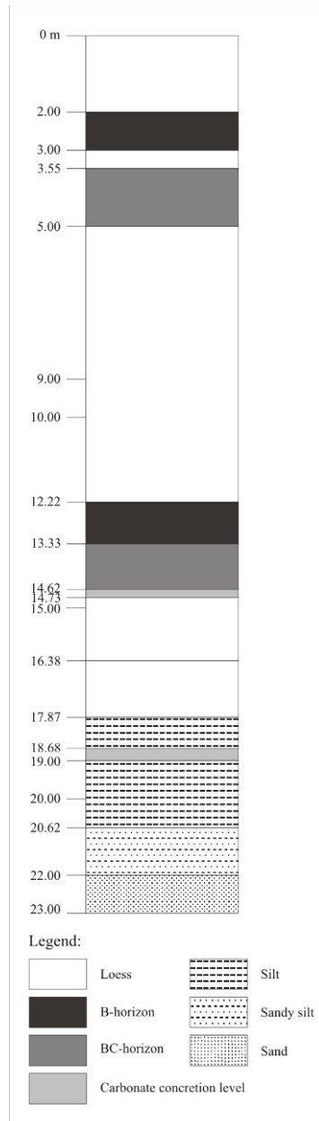
Figure 2. A sketch of the loess profile.
