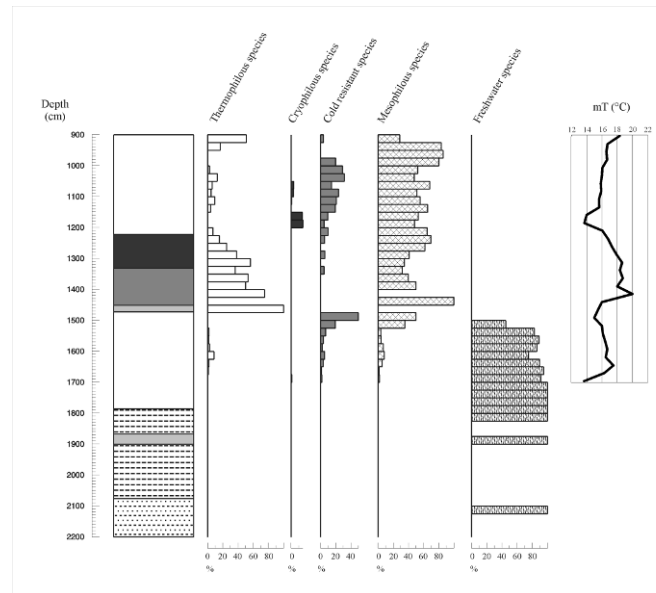
Figure 3. The dominance relationships of the different ecological groups in the mollusc fauna.
