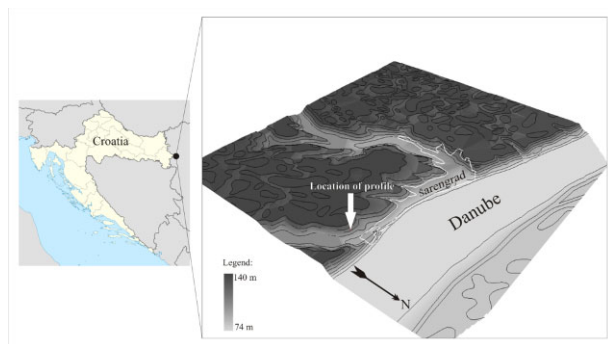
Figure 1. Location of the loess profile at Šaregrad (white line shows the extension of Šaregrad village).
