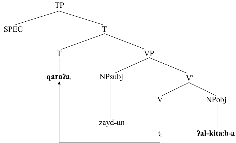
Figure 1. V-to-T movement.
