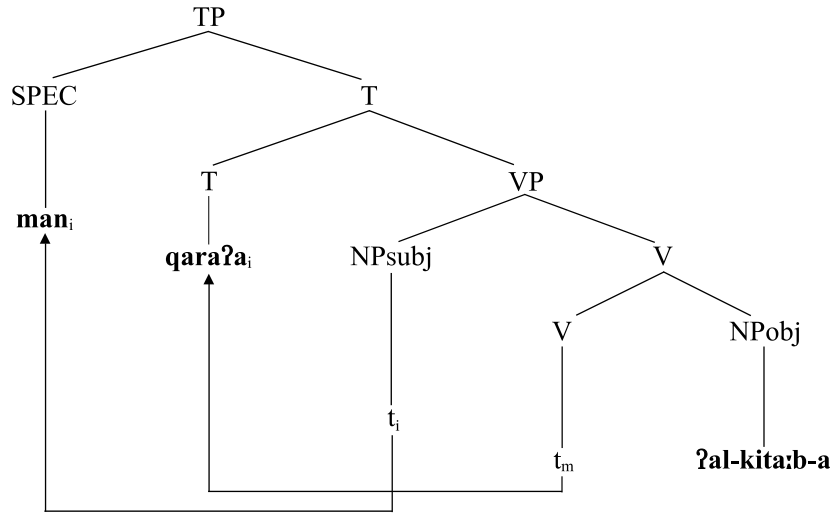
Figure 3. Wh-subject movement.
