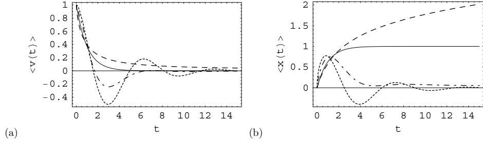
FIGURE 2. Graphical representation in case when \tau \rightarrow 0 , C_{\alpha,\beta,\delta} = 1 , k_B T = 1 , x_0 = 0 , v_0 = 1 of: (a) Mean particle velocity (The following parameters are used: \alpha = \beta = \delta = \mu = 1 (solid line); \alpha = \beta = \delta = \mu = 1/2 (dashed line); \alpha = \delta = 3/4 , \beta = 3/2 , \mu = 1/2 (dot-dashed line); \alpha = \delta = 3/4 , \beta = 3/2 , \mu = 3/4 (dotted line)); (b) Mean particle displacement (The following parameters are used: \alpha = \beta = \delta = \mu = \nu = 1 (solid line); \alpha = \beta = \delta = \mu = 1/2 , \nu = 1 (dashed line); \alpha = \delta = \nu = 3/4 , \beta = 3/2 , \mu = 1/2 (dot-dashed line); \alpha = \delta = \mu = 3/4 , \beta = 3/2 , \nu = 1/2 (dotted line)).
