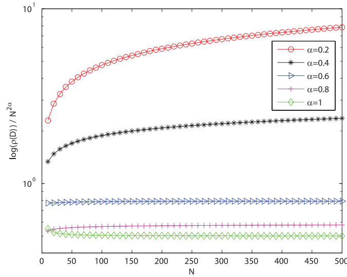
FIGURE 1. The spectral radius associated with the Caputo fractional operator for 0 < \alpha \leq 1 .
