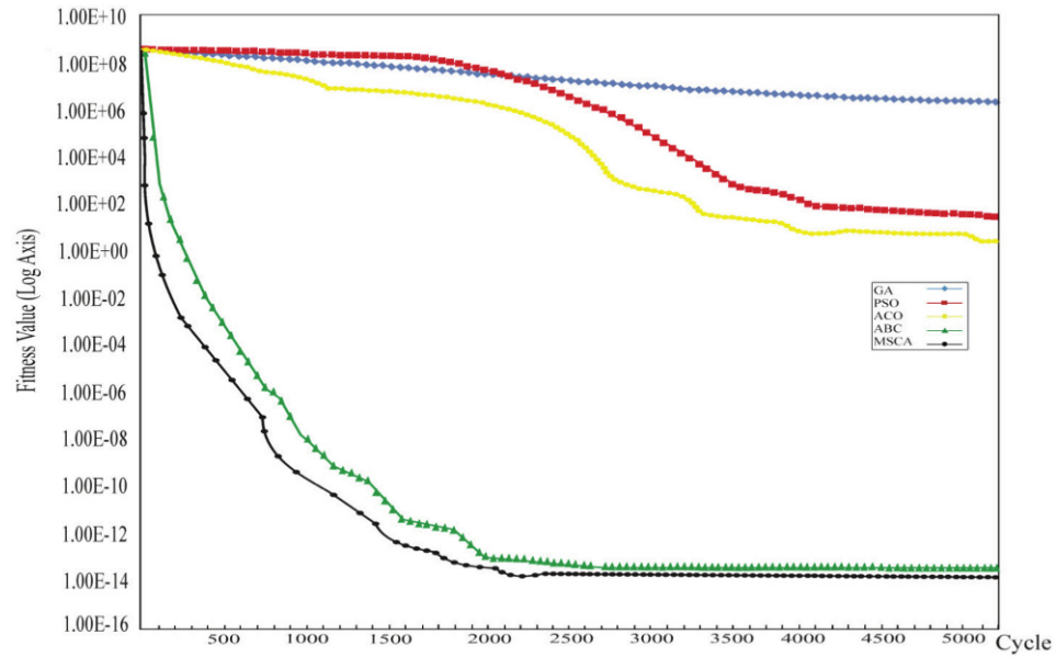
Figure 5. The results of applying different algorithms on Griewank function.
