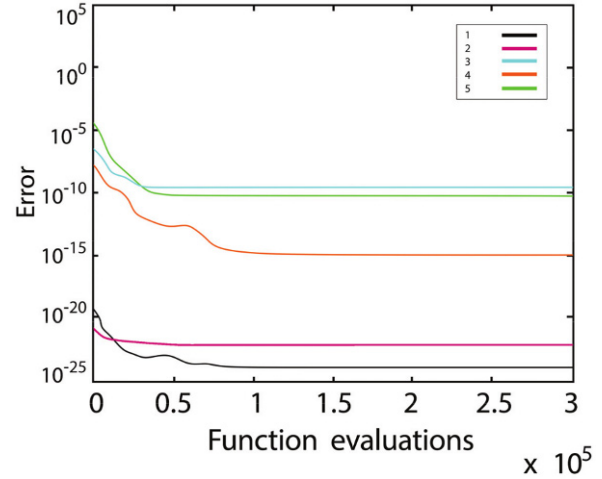
Figure 10. The results of applying the MSCA on F_1 – F_5 (Convergence of Functions F_1 – F_5 ).
