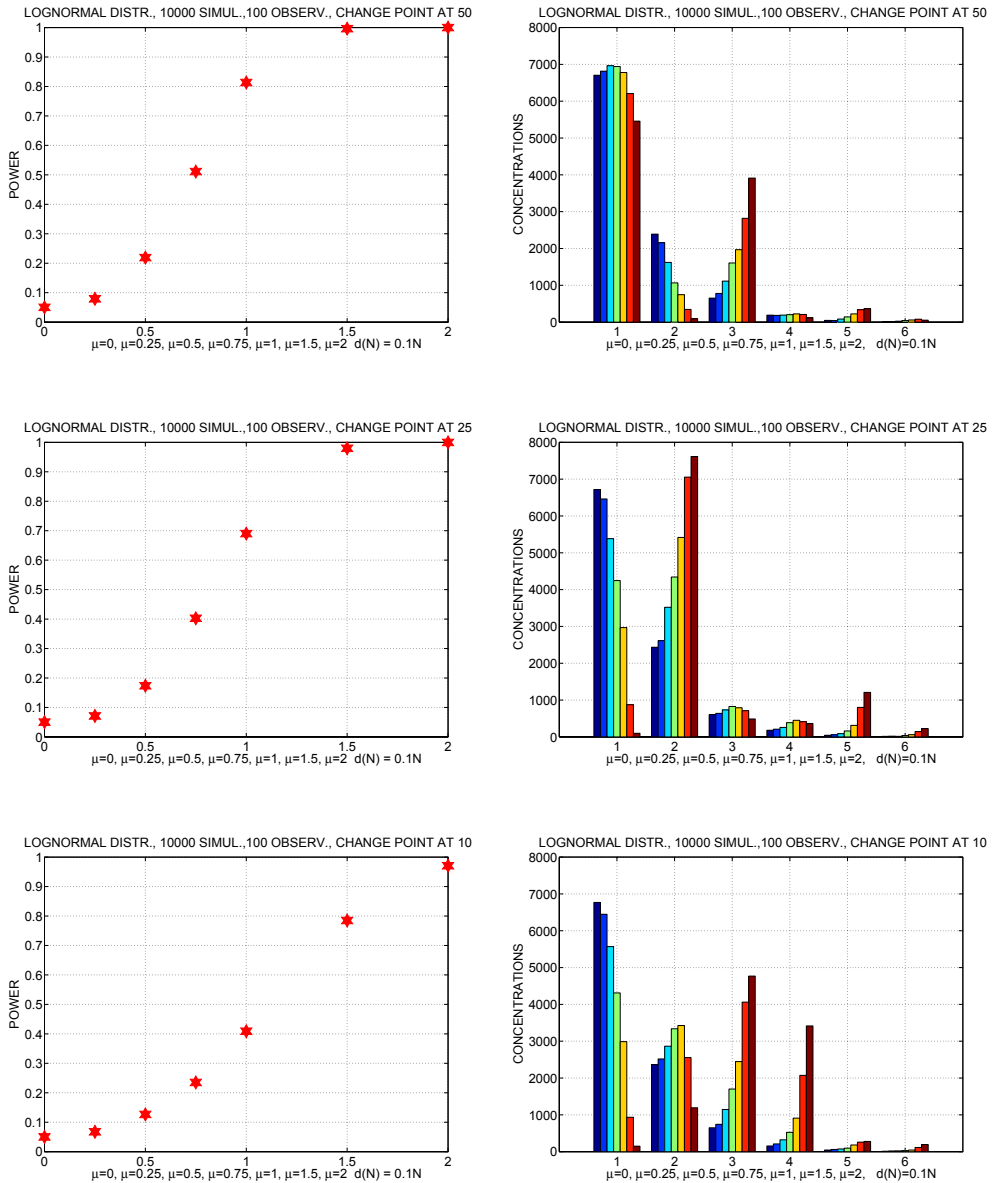
FIGURE 7. Powers of \mathcal{M}_N(0.1; \log N) and concentrations of \tilde{S}(\log N) when changing the parameter \mu of the lognormal distribution.
