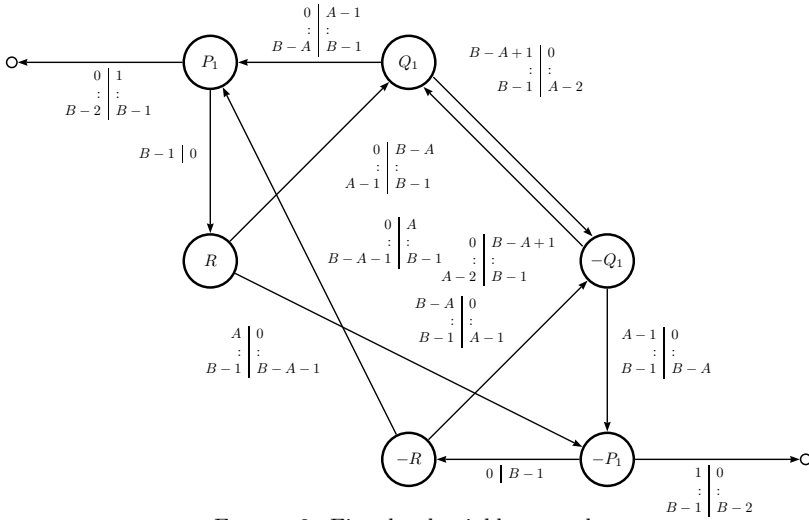
FIGURE 2. First level neighbor graph
