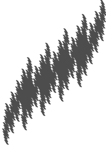
FIGURE 4. A CNS tile with uncountable fundamental group (limit case, with A = 4, B = 5 )
