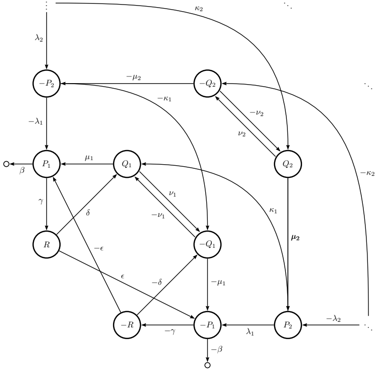
FIGURE 1. General neighbor graph \mathcal{G}_1(\mathcal{S})
