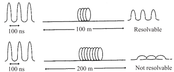
Fig. 2. Pulses separated by 100 ns at the input end may be resolvable at the output end of a 100-m, but not 200-m long fiber.
