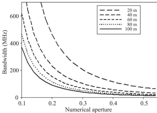
Fig. 4. Bandwidth calculated as a function of the numerical aperture.
