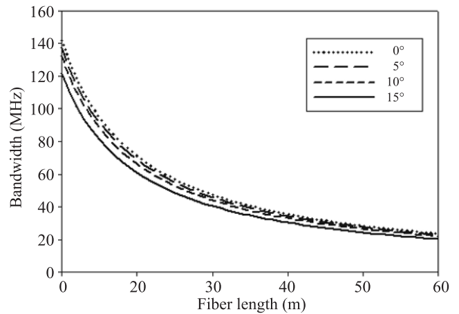
Fig. 9. Bandwidth of SI POF vs. fiber length for several tilt-angles.
