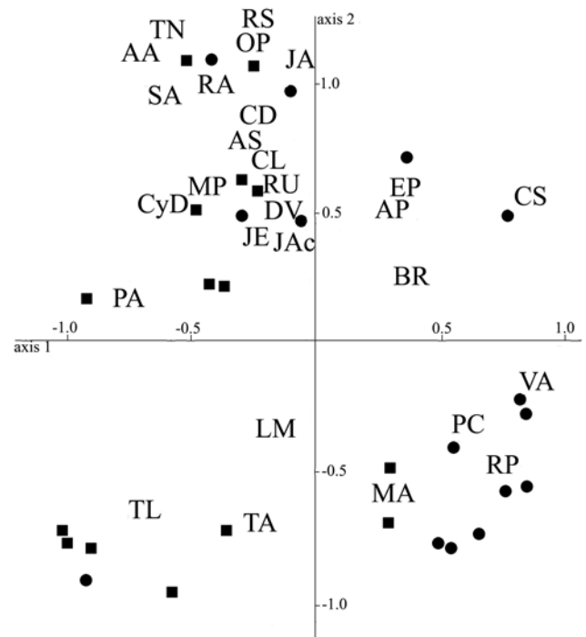
Fig. 3. Distribution of samples and species in the biplot of the NMDS analysis. ● – samples in 2000; ■ – samples in 2009. For the abbreviations of species see Table 2.
