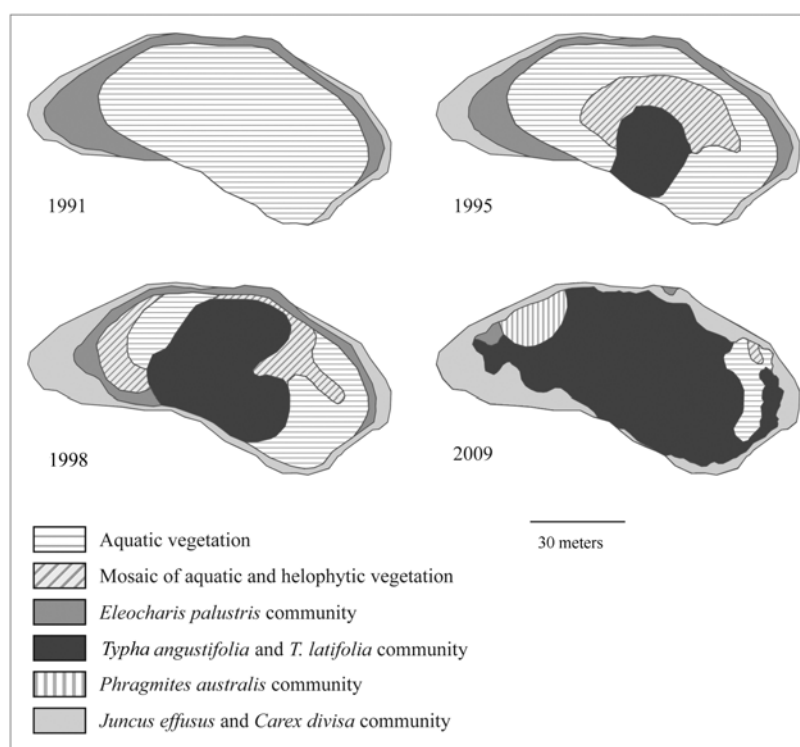
Fig. 2. Vegetation maps of the years studied.
