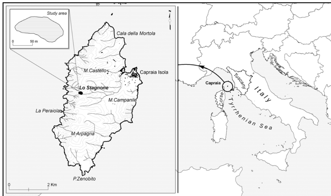
Fig. 1. Study area. Mediterranean Sea with the position of Capraia Island. In the detail Capraia Island with Stagnone Lake is shown.
