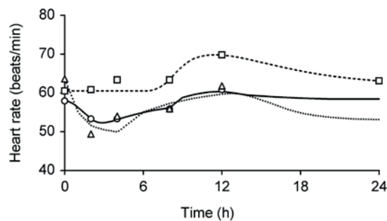
Figure 4. The PK/PD model solution of HR time profile related to measured atenolol (triangles), valsartan (squares) concentrations and their combination (circles).
