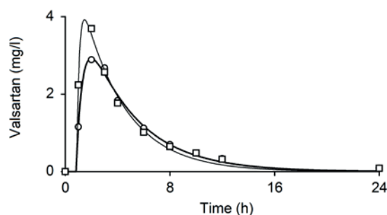
Figure 3. Concentration-time profile of valsartan administered separately and in combination with atenolol by PK model. Squares—measured concentration of valsartan administered separately; circles—measured concentration of valsartan administered in combination with atenolol; line—model approximation.
