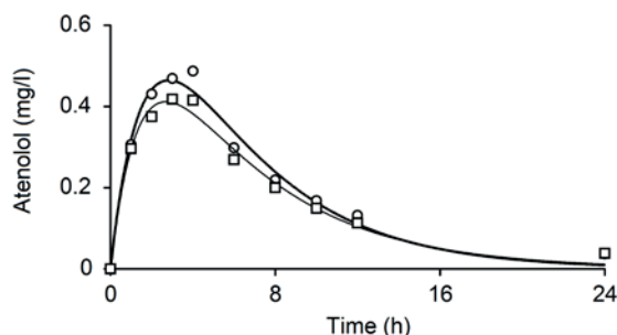
Figure 2. Concentration-time profile of atenolol administered separately and in combination with valsartan by PK model. Squares—measured concentration of atenolol administered separately; circles—measured concentration of atenolol administered in combination with valsartan; line—model approximation.
