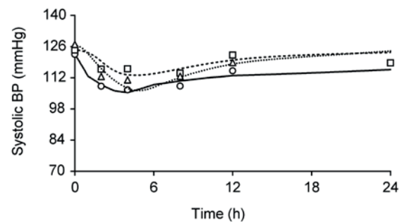
Figure 5. The PK/PD model solution of SP time profile related to measured atenolol (triangles), valsartan (squares) concentrations and their combination (circles).
