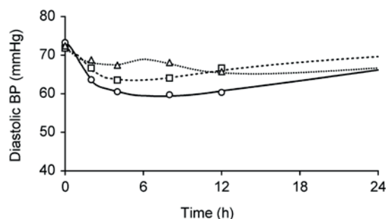
Figure 6. The PK/PD model solution of DP time profile related to measured atenolol (triangles), valsartan (squares) concentrations and their combination (circles).
