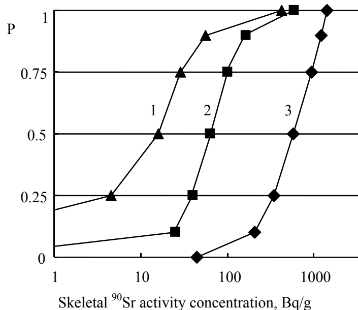
Figure 1. Cumulative distribution of skeletal ^{90}\text{Sr} activity of animals trapped at the territories of EURT with different ^{90}\text{Sr} surface contamination: 1 – 0.074–18.5 MBq/m 2 (n=561); 2 – 18.5–37 MBq/m 2 (n=469); 3 – >37 MBq/m 2 (n=50) [19,29].
