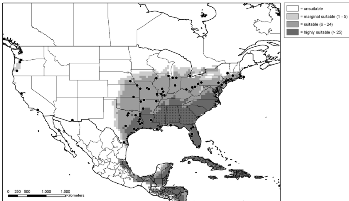
Figure 1. Map of North America showing climatic suitability (ecoclimatic index, EI) for Pueraria lobata using CLIMEX and known distribution of the plant mainly from the periphery for goodness of fit. Known occurrences are shown as a point location or at the county level (●). In highly climatically suitable areas (EI > 25), Pueraria lobata may occur abundant and damaging. The states of Alabama, Georgia and Mississippi are stippled to indicate the area with the heaviest infestations of Pueraria lobata .
