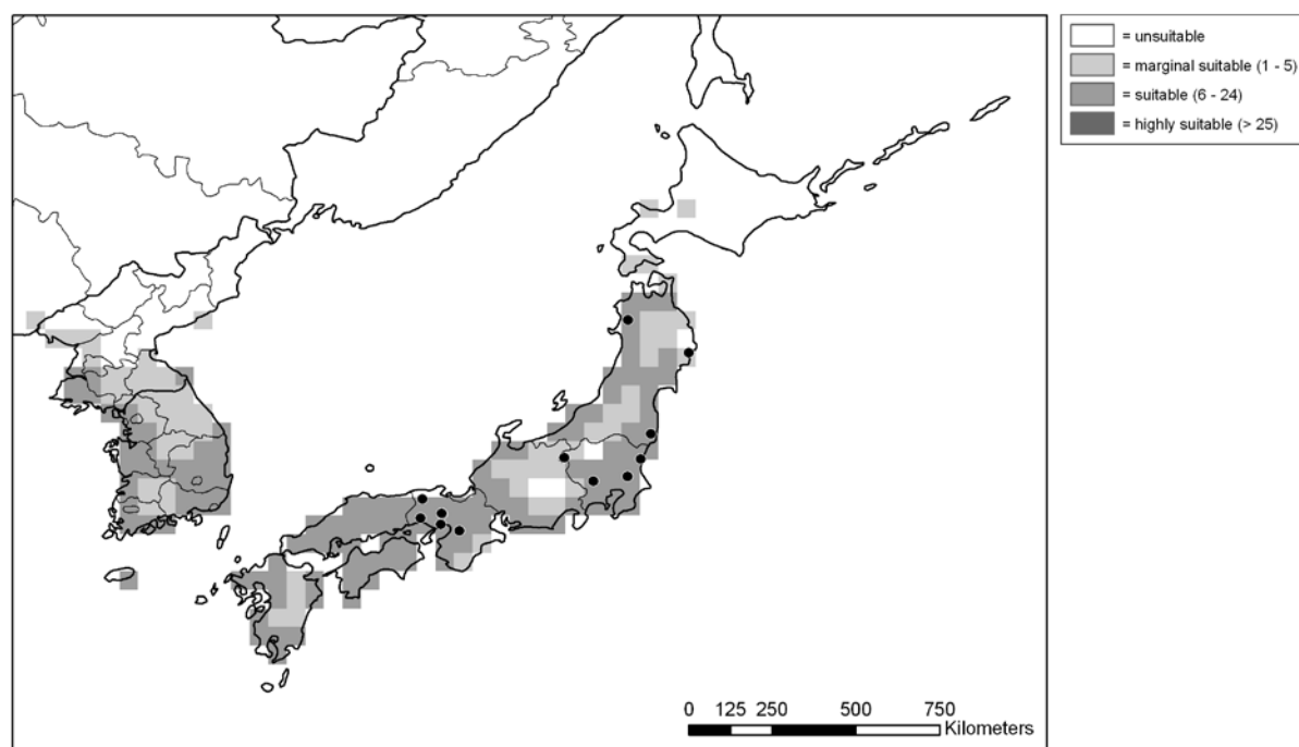
Figure 2. Map of Japan showing climatic suitability (ecoclimatic index, EI) for Pueraria lobata using CLIMEX and known distribution of the plant for goodness of fit. Known occurrences are shown as a point location (●).
