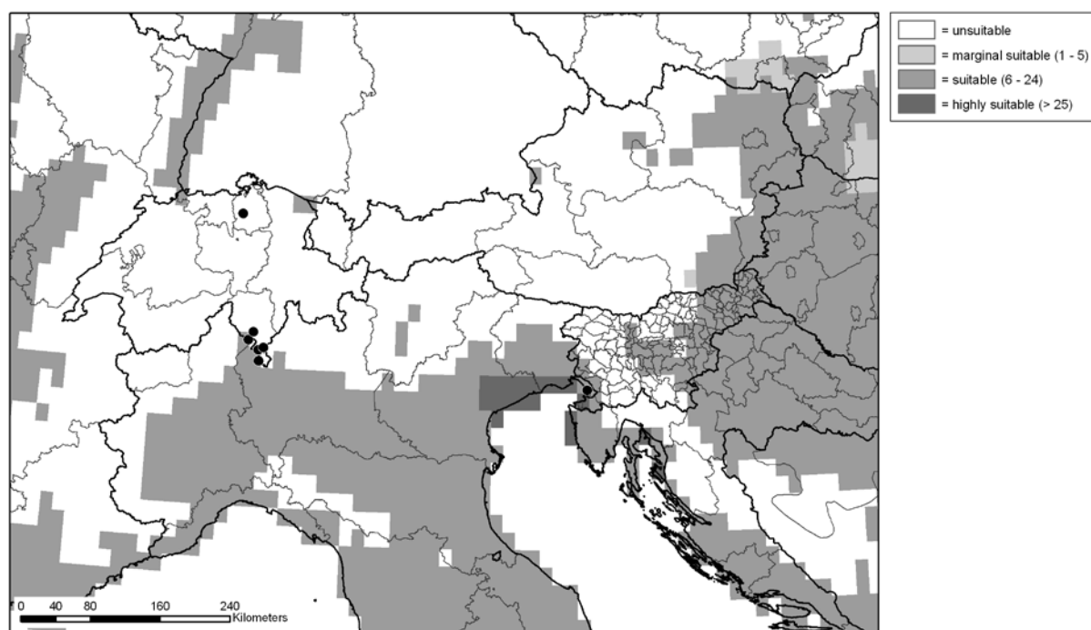
Figure 3. Map of Austria, Switzerland, Slovenia, northern Italy and neighbouring countries showing climatic suitability (ecoclimatic index, EI) for Pueraria lobata using CLIMEX and known distribution (●) of the plant for goodness of fit. Known occurrences are shown as a point location (●). In highly climatically suitable areas (EI > 25), Pueraria lobata may occur abundant and damaging.
