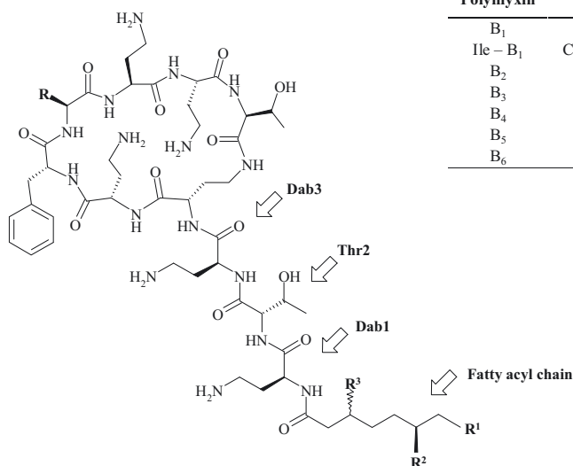
Figure 2. General structure for polymyxin B. Polymyxin B is a complex constituted of six members, differing in fatty acyl chain and in amino acid identity at position 7 of the cyclic portion (R substituents are reported in table). The arrows point out the sites modified to obtain NAB7061 and NAB739 polymyxin B derivatives. Both derivatives lack the Dab1 residue and bear an uncharged amino acid at position 3 instead of the charged Dab3. The NAB739 linear peptide portion is constituted of Thr-D-Ser and that of NAB7061 is constituted of Thr-Abu, reducing the overall number of charges from 5 to 3.
