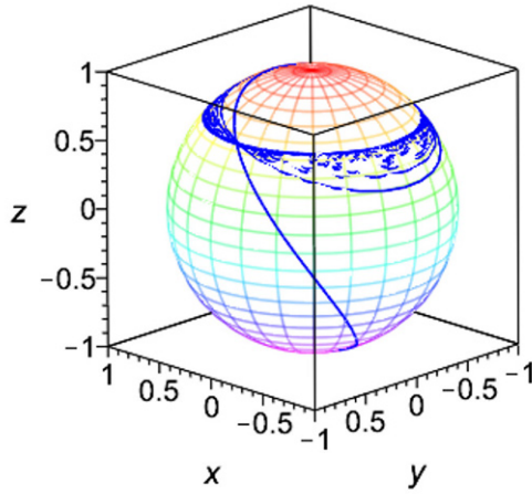
Figure 1. (Color online) Bloch vector's dynamics. The evolution starts at the south pole of the sphere. Top panel: ( \omega = 3 ). Bottom panel: \omega = 0.75 .
