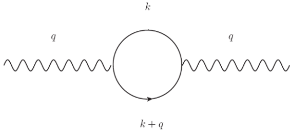
Figure 1. 1-loop vacuum polarization diagram.
