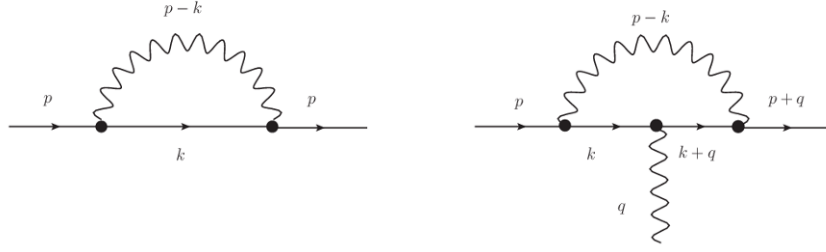
Figure 2. 1-loop diagrams for the Ward identity.
