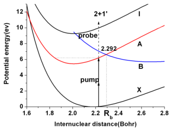
Figure 1. The NO potential curves employed in our calculation [20–24, 29]
