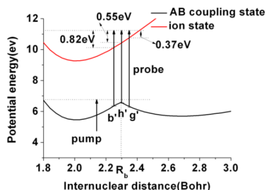
Figure 4. Potential line of the AB coupled state. The letters g', h' and b' represent three vibrational states of the coupled excited state.
