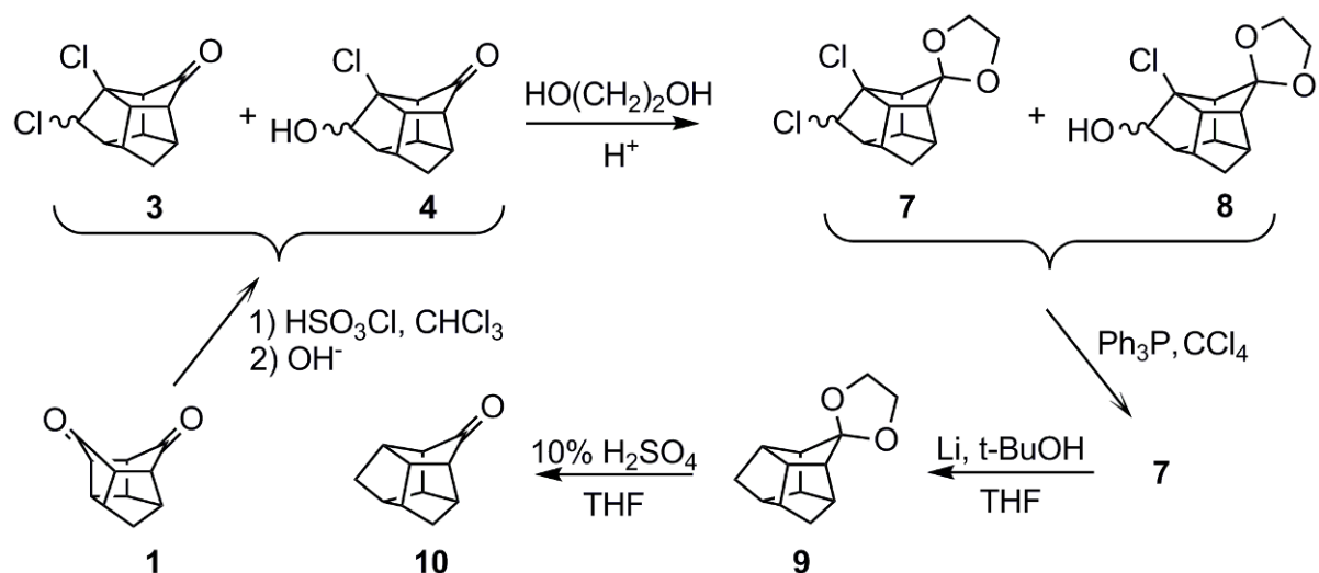
Scheme 2. Multigram synthesis of D 3 -trishomocubanone ( 10 ).
