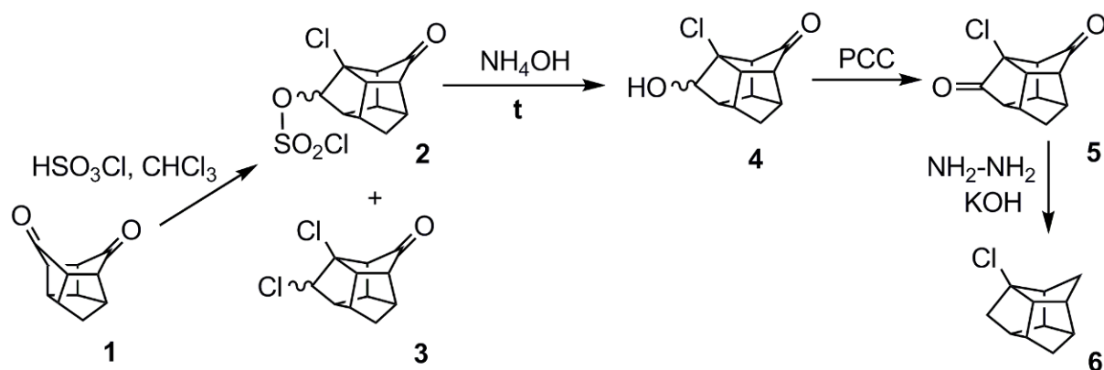
Scheme 1. Chlorosulfonation of Cookson's diketone ( 1 ).
