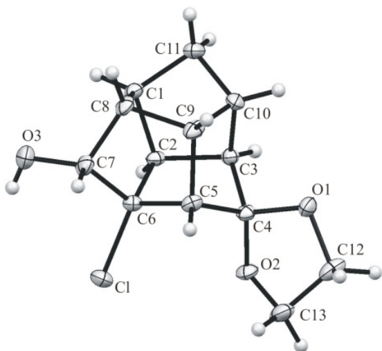
Figure 1. The X-ray crystal structure of 6-chloro-7-hydroxypentacyclo[6.3.0.0 2,6 .0 3,10 .0 5,9 ]undecane-4-one ethylene ketal ( 8 ).
