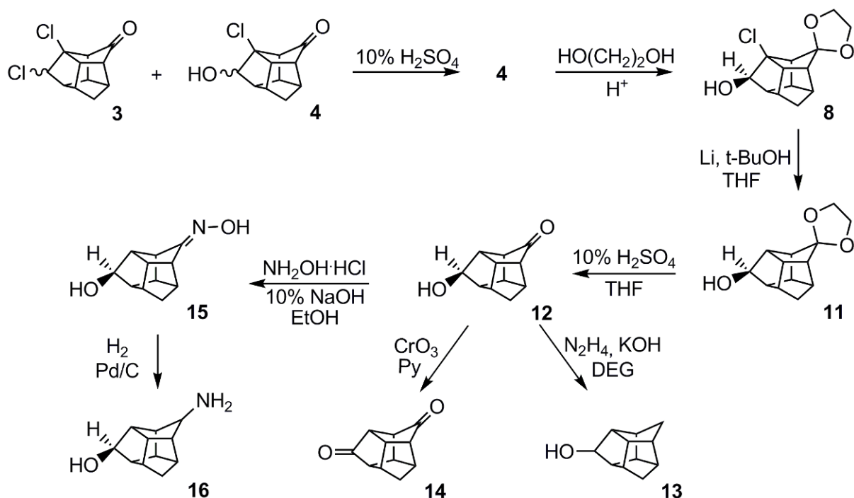
Scheme 3. Preparation of individual epimers of 4,7-disubstituted D_3 -trishomocubane derivatives.
