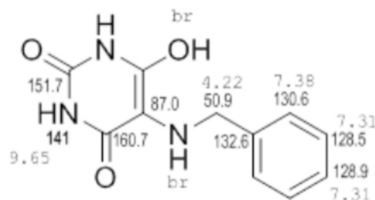
Figure 1. Structure determination for C5-amino barbiturate 4a with gHMBC experiment.
