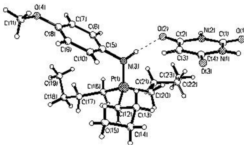
Figure 2. Molecular structure of 6f according to an X-ray diffraction study.
