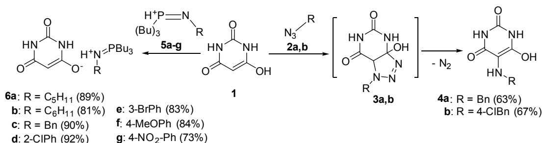
Scheme 1. Synthesis of C5-amino barbiturates 4a-b and tributylphosphoranylidene salts of BA 6a-g .
