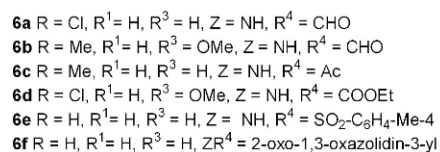
Scheme 2. Exploitation of 3 for the synthesis of 5-substituted 3-(2-oxo-2H-chromen-3-yl)-2H,5H-pyrano[3,2-c]chromene derivatives 4-6 .
