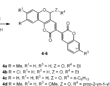
Scheme 2. Exploitation of 3 for the synthesis of 5-substituted 3-(2-oxo-2H-chromen-3-yl)-2H,5H-pyrano[3,2-c]chromene derivatives 4-6 .
