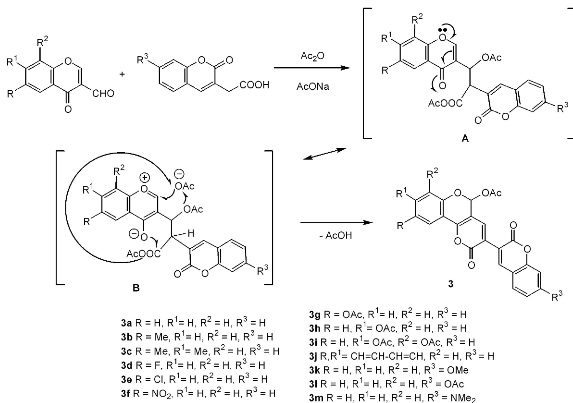
Scheme 1. Synthesis of 3-(2-oxo-2H-chromen-3-yl)-2-oxo-2H,5H-pyrano[3,2-c]chromen-5-yl acetates 3 .
