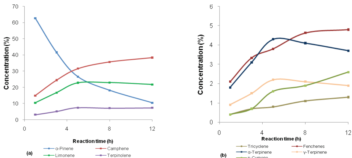
Figure 5. (a) Concentration of the major products in the reaction mixture depending on the reaction time for \text{H}_4\text{SiW}_{12}\text{O}_{40}/\text{SiO}_2 catalyst ( \alpha -pinene/catalyst ratio of 100/1, at 100°C); (b) Concentration of the minor products in the reaction mixture depending on the reaction time for \text{H}_4\text{SiW}_{12}\text{O}_{40}/\text{SiO}_2 catalyst ( \alpha -pinene/catalyst ratio of 100/1, at 100°C)
