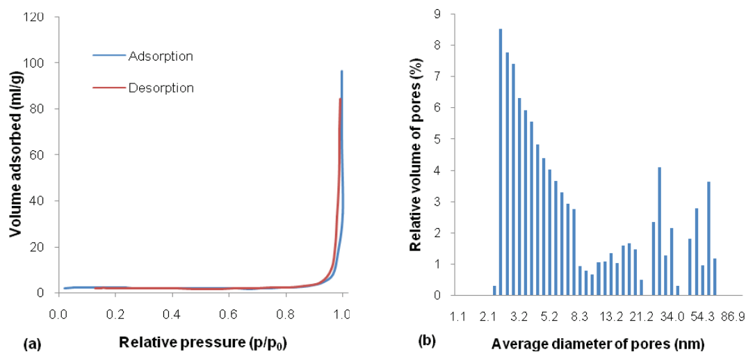
Figure 2. (a) Nitrogen adsorption/desorption isotherms at 77 K; (b) Pore size distribution of \text{H}_4\text{SiW}_{12}\text{O}_{40}/\text{TiO}_2 catalyst.
