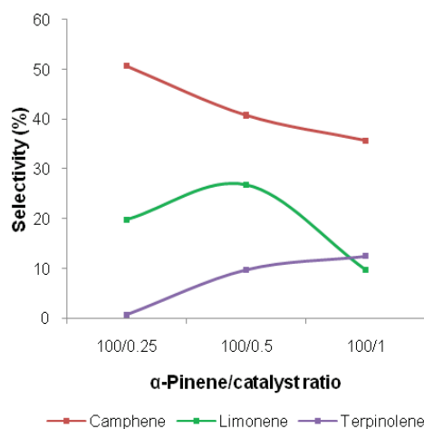
Figure 8. Effect of the catalyst concentration on the selectivity of camphene, limonene and terpinolene at 130°C, using H_4SiW_{12}O_{40}/SiO_2 catalyst.
