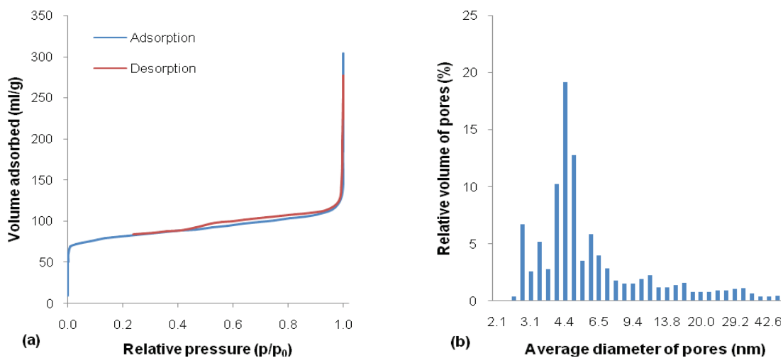
Figure 3. (a) Nitrogen adsorption/desorption isotherms at 77 K; (b) Pore size distribution of \text{H}_4\text{SiW}_{12}\text{O}_{40}/\text{HZSM-5} catalyst.
