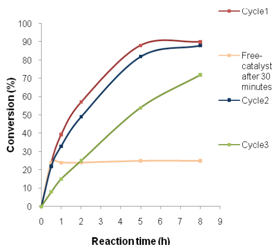
Figure 10. Kinetic curves for three recovery/reutilization cycles and the effect of the SiW leaching for H_4SiW_{12}O_{40}/SiO_2 catalyst ( \alpha -pinene/catalyst ratio of 100/1, at 100°C).
