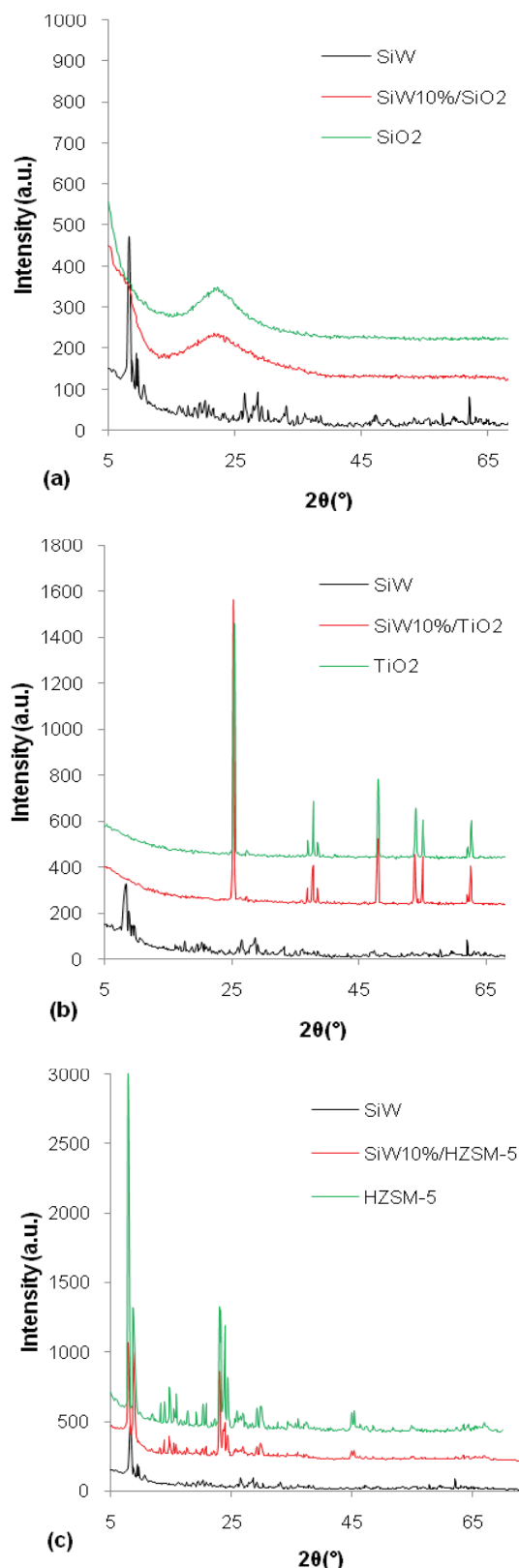
Figure 4. PXRD patterns for: (a) SiW, SiW10%/SiO 2 , SiO 2 ; (b) SiW, SiW10%/TiO 2 , TiO 2 ; (c) SiW, SiW10%/HZSM-5, HZSM-5.
