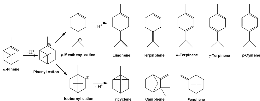
Scheme 1. Acid-catalyzed isomerization of \alpha -pinene.
