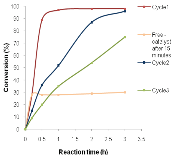
Figure 11. Kinetic curves for three recovery/reutilization cycles and the effect of the SiW leaching for \text{H}_4\text{SiW}_{12}\text{O}_{40} /HZSM-5 catalyst ( \alpha -pinene/catalyst ratio of 100/1, at 160^\circ\text{C} ).
