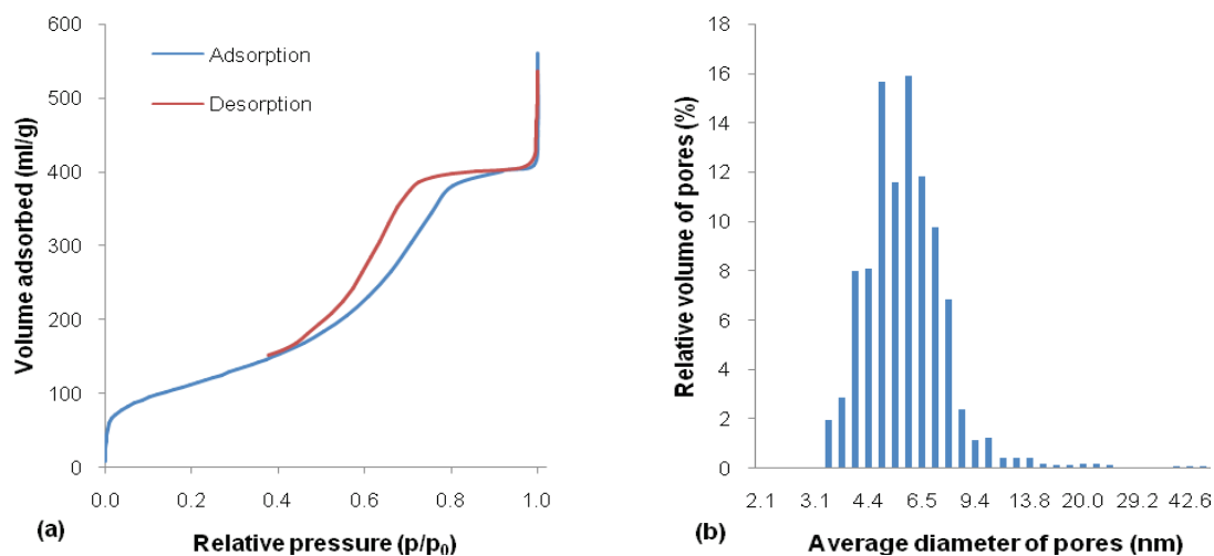
Figure 1. (a) Nitrogen adsorption/desorption isotherms at 77 K; (b) Pore size distribution of \text{H}_4\text{SiW}_{12}\text{O}_{40}/\text{SiO}_2 catalyst.
