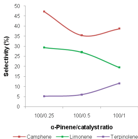
Figure 9. Effect of the catalyst concentration on the selectivity to camphene, limonene and terpinolene (160°C, H_4SiW_{12}O_{40}/HZSM-5 ).
