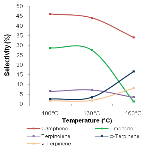
Figure 7. Effect of the reaction temperature on the selectivity of camphene, limonene and terpinolene ( \alpha -pinene/catalyst: 100/1, \text{H}_4\text{SiW}_{12}\text{O}_{40}/\text{TiO}_2 as a catalyst).
