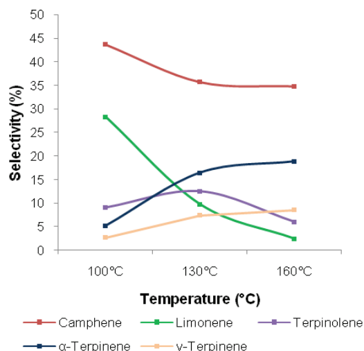
Figure 6. Effect of the reaction temperature on the selectivity of camphene, limonene and terpinolene ( \alpha -pinene/catalyst: 100/1, catalyst \text{H}_4\text{SiW}_{12}\text{O}_{40}/\text{SiO}_2 )
