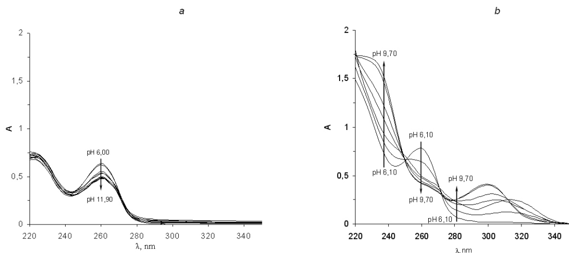
Figure 2. UV spectra of the adduct of 3-PBA (22 mg/l) with CH 3 I at different pH in water (a) and in the presence of 0.5 mM H 2 O 2 (b); 1 M KCl; water, 25°C.
