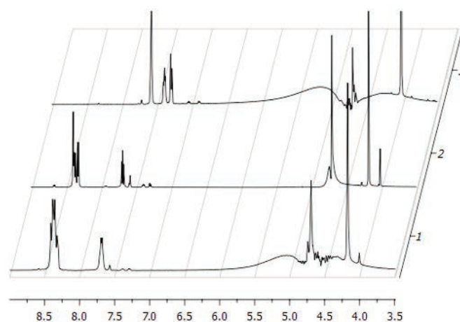
Figure 4. ^1\text{H} NMR ( \text{H}_2\text{O} - \text{D}_2\text{O} mixture, 25^\circ\text{C} , water suppression) spectra of 3a iodide (0.01 M phosphate buffer solution) in the presence of 10-fold excess of \text{H}_2\text{O}_2 vs time: 2 h (bottom line); 72 h (medium line); 1-methyl-3-hydroxyl pyridinium iodide (upper spectrum).
