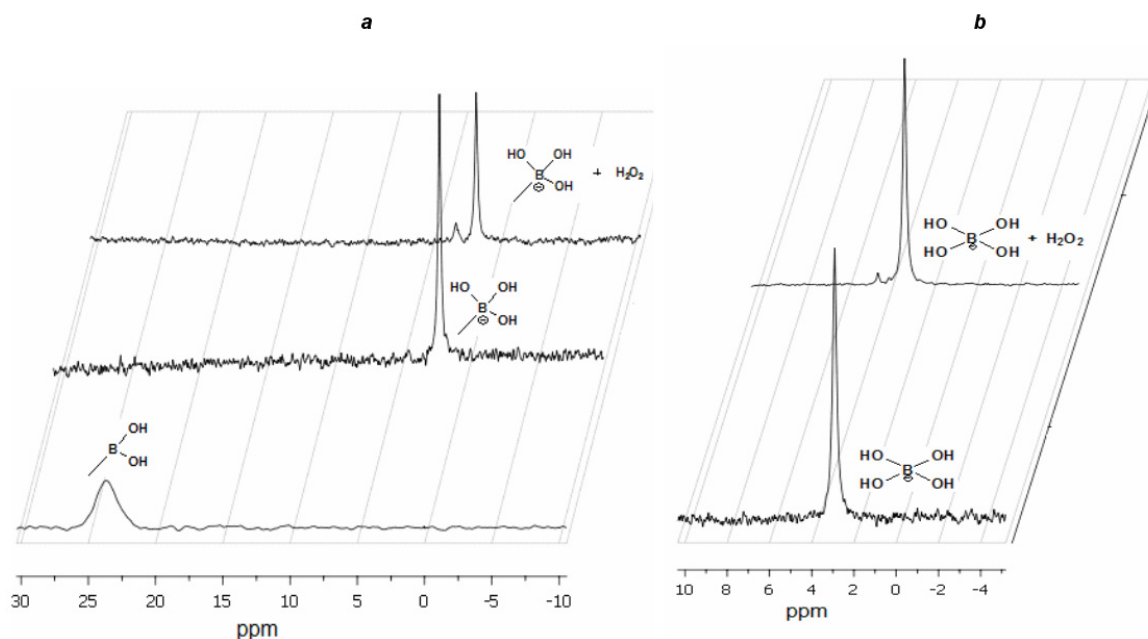
Figure 5. ^{11}\text{B} NMR ( \text{H}_2\text{O} - \text{D}_2\text{O} mixture, \text{BF}_3\text{OEt}_2 is a reference) spectra of (a) 3a iodide and (b) boric acid in the presence and absence of hydrogen peroxide, pH 10.0; 0.01 M phosphate buffer solution. The bottom spectrum in (a) corresponds to pH 3.3.
