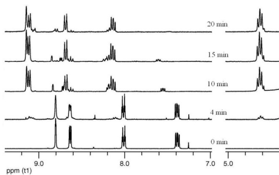
Figure 3. 1 H NMR (DMSO-d 6 ) spectra for the reaction of 1 with iodododecane at different times of microwave irradiation (300 W).
