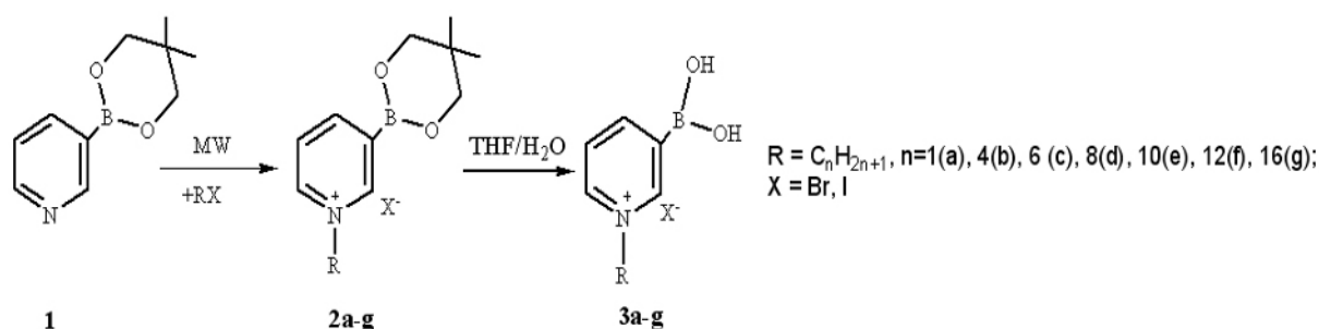
Figure 1. Scheme for N -alkyl-3-boronopyridinium halide preparation using microwave irradiation.
