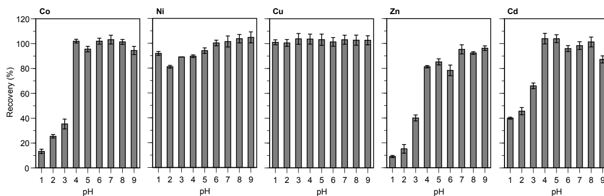
Figure 2. Effect of pH on the collection behavior of the MRT-SPE column. Sample solution: 250 \mu\text{g L}^{-1} (Co, Ni, Cu, Zn or Cd), pH: 1–9, volume: 4 mL, loading flow rate: 1 \text{ mL min}^{-1} , eluent: 3 M \text{HNO}_3 , eluent volume: 4 mL, elution flow rate: 1 \text{ mL min}^{-1} ( n = 3 ).
