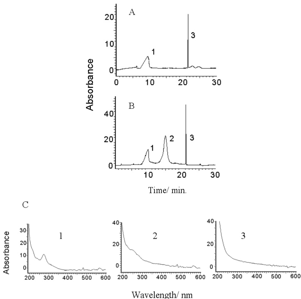
Figure 2. CZE separation of charged QDs: CdSe/ligand and CdSe/ligand 1 /ligand 2 . Frames: A, 1 CdSe/DHLA, 3 CdSe/(PhSO 3 ) 2 phen; B, peaks 1, 3 the same as in frame A; 2, CdSe/(PhSO 3 ) 2 phen/DHLA; C, spectra of peaks of CdSe QDs. Conditions: background buffer, 20 mM potassium chloride; pH 6.0; voltage 20 kV ( \rightarrow 44 \mu A). All QDs were synthesized from CdSe/TOP, size 3.2 nm.
