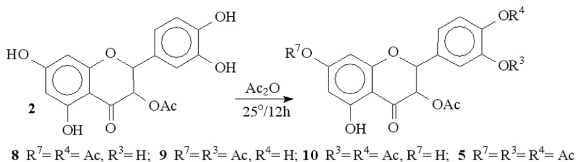
Scheme 2. Acetylation of 2 .
