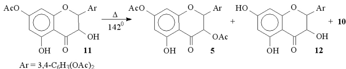
Scheme 3. Transacylation of 11 .
