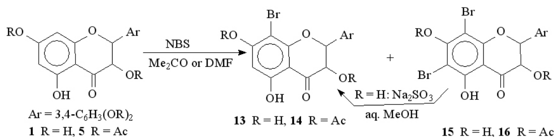
Scheme 4. Bromination of dhq and dhqAc373'4' .
