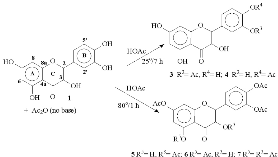
Scheme 1. Acetylation of 1 .
