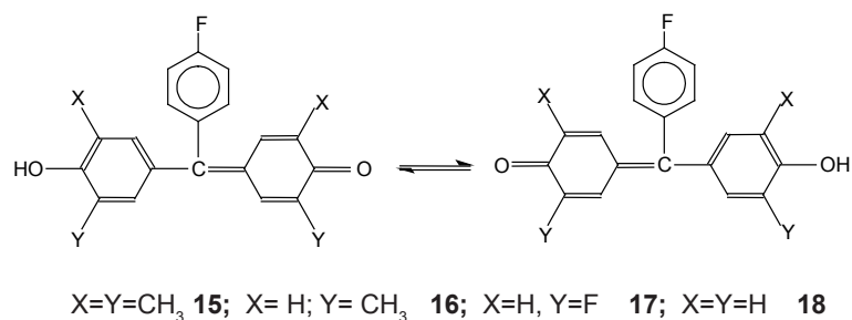
Figure 4. Tautomers of 15 - 18
