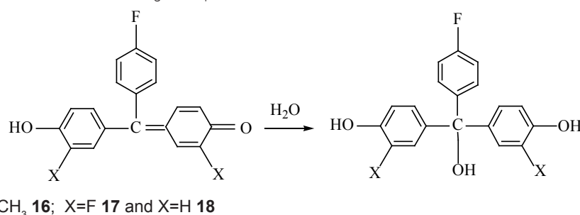
Figure 1. Tautomeric scheme and numbering of compounds
