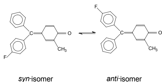
Figure 3. Syn - and anti -isomers as illustrated by 10 .
