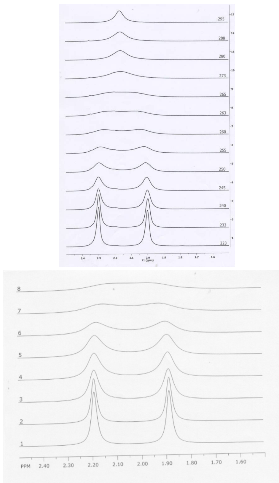
Figure 8. ^1\text{H} spectrum of 15 with 2.5 moles of water added; (a) experimental traces, (b) simulated traces for temperatures from 223 K to 263 K.
