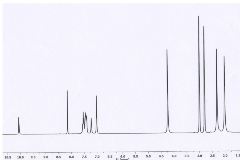
Figure 7. 1 H spectrum of 15 at -50°C.
