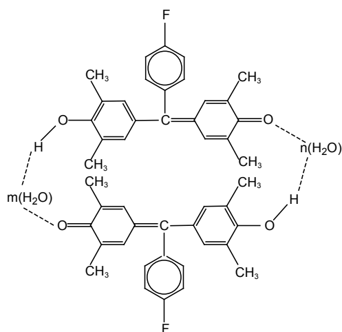
Figure 5. Water catalysis model involving two molecules of 15 .
