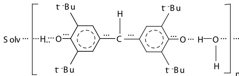
Figure 6. Hydroxygalvinoxyl and suggested three component system from [4]
