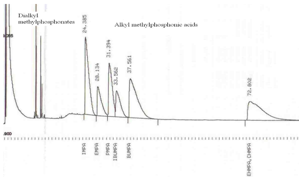
Figure 3. GC FID chromatogram of a mixture of alkyl methylphosphonic acids (samples injected in acetone (1 \mu L), column CP-FFAP CB, temperature program: 50°C (5 min) \rightarrow 190°C (10°C min -1 ) \rightarrow 190°C; helium flow 7.2 mL min -1 , injector temperature 230°C, detector (FID) temperature 270°C; concentration of analyzed compounds [mg mL -1 ]: IMPA – 0.91, EMPA – 0.44, PMPA – 0.58, IBUMPA – 0.36, BUMPA – 0.98, EHMPA – 0.92, CHMPA – 0.59.
