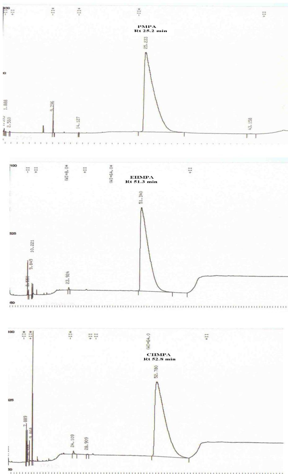
Figure 2. GC FID chromatograms of alkyl methylphosphonic acids: 1. EMPA, 2. IMPA, 3. IBUMPA, 4.PMPA, 5. EHMPA, 6. CHMPA; GC performed on column CP-FFAP CB, temperature program: 50°C (5 min) \nearrow 190°C(10°C min -1 ) \nearrow 190°C (15 min for IMPA, 25 min for EMPA, PMPA and IBUMPA, 50 min for EHMPA and CHMPA) \nearrow 230°C (10°C min -1 ), helium flow 22 mL min -1 , injector temperature 230°C, detector (FID) temperature 270°C.
