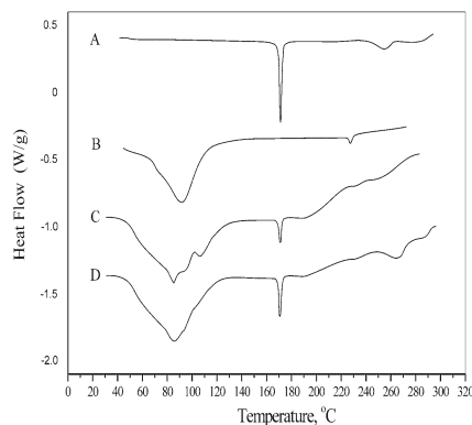
Figure 6. DSC curves of (A) nifedipin, (B) \beta -cyclodextrin, the inclusion complex of nifedipin and (C) \beta -cyclodextrin and (D) the physical mixture of nifedipin and \beta -cyclodextrin
