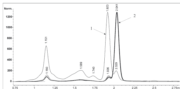
Figure 7. HPLC chromatogram of nifedipin: (1) nitro-derivative of nifedipin without irradiation, (2) nitroso-derivative of nifedipin obtained by irradiation at 350 nm for 5, 10, 15, 20, 25 and 30 min.
