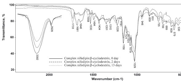
Figure 10. FTIR spectra of nifedipin complex with \beta -cyclodextrin exposed to daylight for several days
