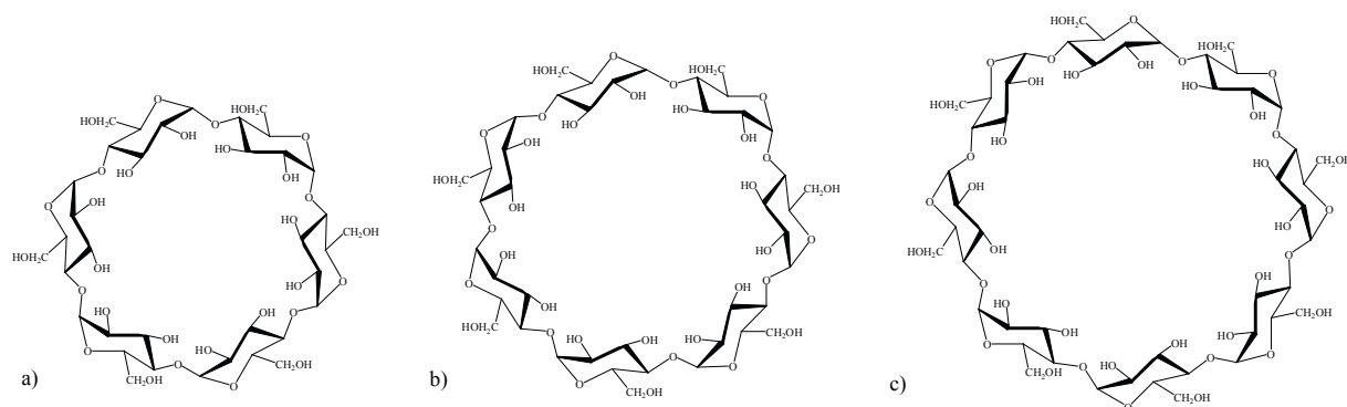
Figure 2. Structures of cyclodextrins: a) \alpha -cyclodextrin, b) \beta -cyclodextrin, and c) \gamma -cyclodextrin
