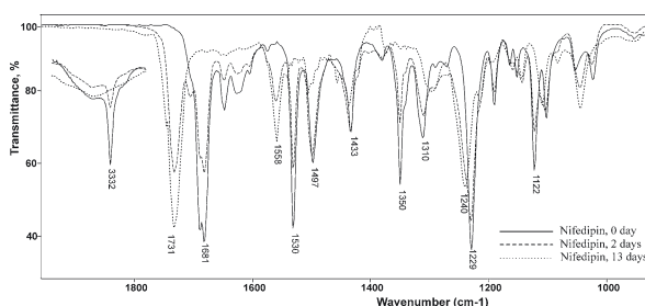
Figure 9. FTIR spectra of nifedipin exposed to daylight for several days
