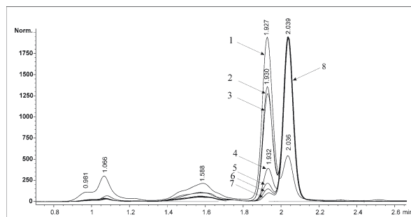
Figure 8. HPLC chromatogram of nifedipin and \beta -cyclodextrin complex: nitro-derivative of (1) nifedipin complex without irradiation, (2) products after complex irradiation at 350 nm for 5 min; (3) 10 min; (4) 15 min; (5) 20 min; (6) 25 min; (7) 30 min and (8) nitroso-derivative of nifedipin from complex.
