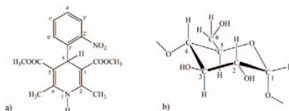
Figure 4. (a) Nifedipin molecule and (b) glucopyranose unit with indicated protons which give signals in 1 H-NMR spectra
