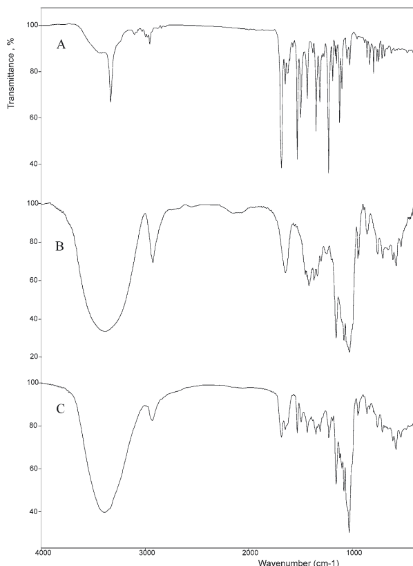
Figure 5. FTIR spectra of (A) nifedipin, (B) \beta -cyclodextrin and (C) the inclusion complex of nifedipin and \beta -cyclodextrin.
