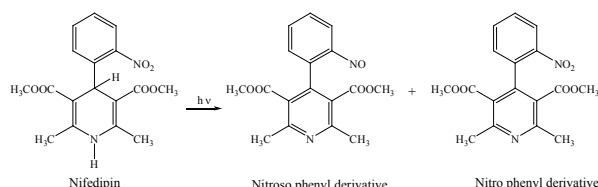
Figure 1. Nifedipin degradation under the influence of light to nitroso derivatives [4-(2-nitrosophenyl)-2,6-dimethyl-3,5-dimethoxy carbonyl pyridine] and nitro derivative [4-(2-nitrophenyl)-2,6-dimethyl-3,5-dimethoxy carbonyl pyridine].
