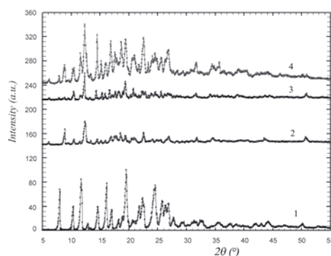
Figure 3. X-ray diffractograms of (1) nifedipin, (2) \beta -cyclodextrin, inclusion complex of nifedipin and (3) \beta -cyclodextrin, and (4) physical mixture of nifedipin and \beta -cyclodextrin
