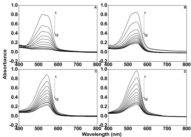
Figure 2. Spectral change of 0.050 mmol L -1 ACBK (A) and 0.050 mmol L -1 ACBK with 0.0100, 0.0200 and 0.0300 mmol L -1 Cu 2+ (B, C and D) at pH 5.0 buffer solutions with 0.05% P25 TiO 2 and UV-light at given time intervals. Spectra from 1 to 12 denote irradiation times from 0 to 55 min with 5 min intervals
