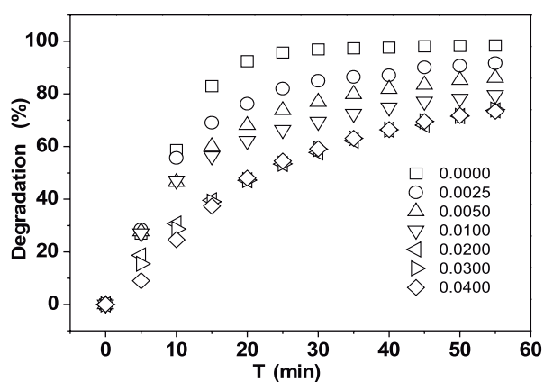
Figure 3. The degradation of 0.050 mmol L -1 ACBK with controlled Cu 2+ concentrations (0.000, 0.0025, 0.0050, 0.0100, 0.0200, 0.0300 and 0.0400 mmol L -1 ) at pH 5.0 buffer solution with 0.05% P25 TiO 2 and UV-light at different times.
