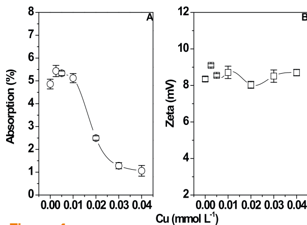
Figure 4. The adsorption of ACBK on the surface of P25 TiO 2 (A) and the change of Zeta potential of P25 TiO 2 (B) at different concentration of Cu 2+ .
