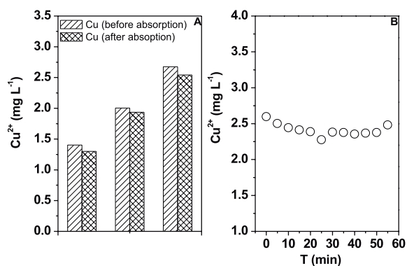
Figure 5. The adsorption of Cu 2+ on P25 TiO 2 (A) and the change of Cu 2+ concentration during the irradiation time (B).
