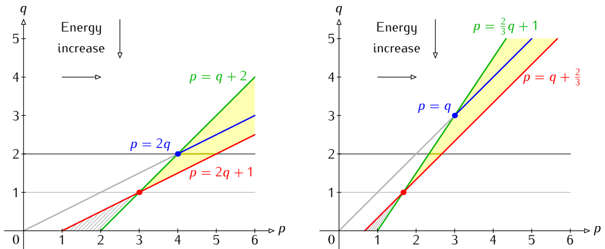
Fig. 3. The ranges of the tangent-point energies (left) and the integral Menger curvature (right). Above the green line, the functionals are not self-repulsive; below the red line, they are highly singular. The yellow area marks the sub-critical range, the dark yellow line the non-degenerate sub-critical range, cf. Fig. 2. The blue line indicates the “classical” energy functionals investigated by Strzelecki et al. [26, 27]. The functionals \text{TP}^{(p,q)} and \text{intM}^{(p,q)} correspond to \text{KE}^{(s,\varrho)} where s = \frac{p-1}{q} or s = \frac{3p-2}{q} - 1 respectively and \varrho = q , see [6, 8] for details.
