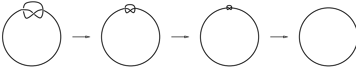
Fig. 1. The pull-tight phenomenon.
