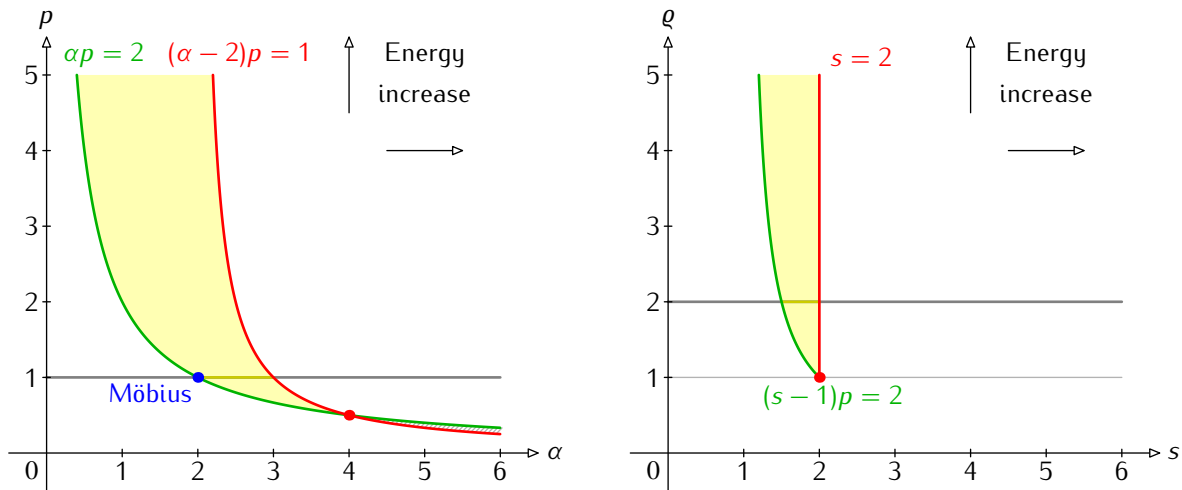
Fig. 2. The range of O'Hara's energies (left); the range of abstract energies (right). On the left-hand side we depict the situation of O'Hara's energies O'H^{(\alpha, p)} . Below the green curve, the respective functionals are not self-repulsive, thus no knot energies. On and above the red line the functionals are so singular that they only take the value infinity. The yellow area between the two curves marks the sub-critical range for which we prove self-repulsiveness and existence of minimizers in every knot class. The darker yellow line \alpha \in (2, 3) , p = 1 denotes the non-degenerate sub-critical range where local minimizers are C^\infty . Any functional O'H^{(\alpha, p)} corresponds to the abstract functional KE^{(s, q)} where s = \frac{\alpha}{2} - \frac{1}{2p} + 1 and q = 2p . The respective parameter ranges are shown on the right-hand side. The energy increase does not follow from the axioms (K_1) , (K_2) , (K_3) , but applies for the examples discussed in this section.
