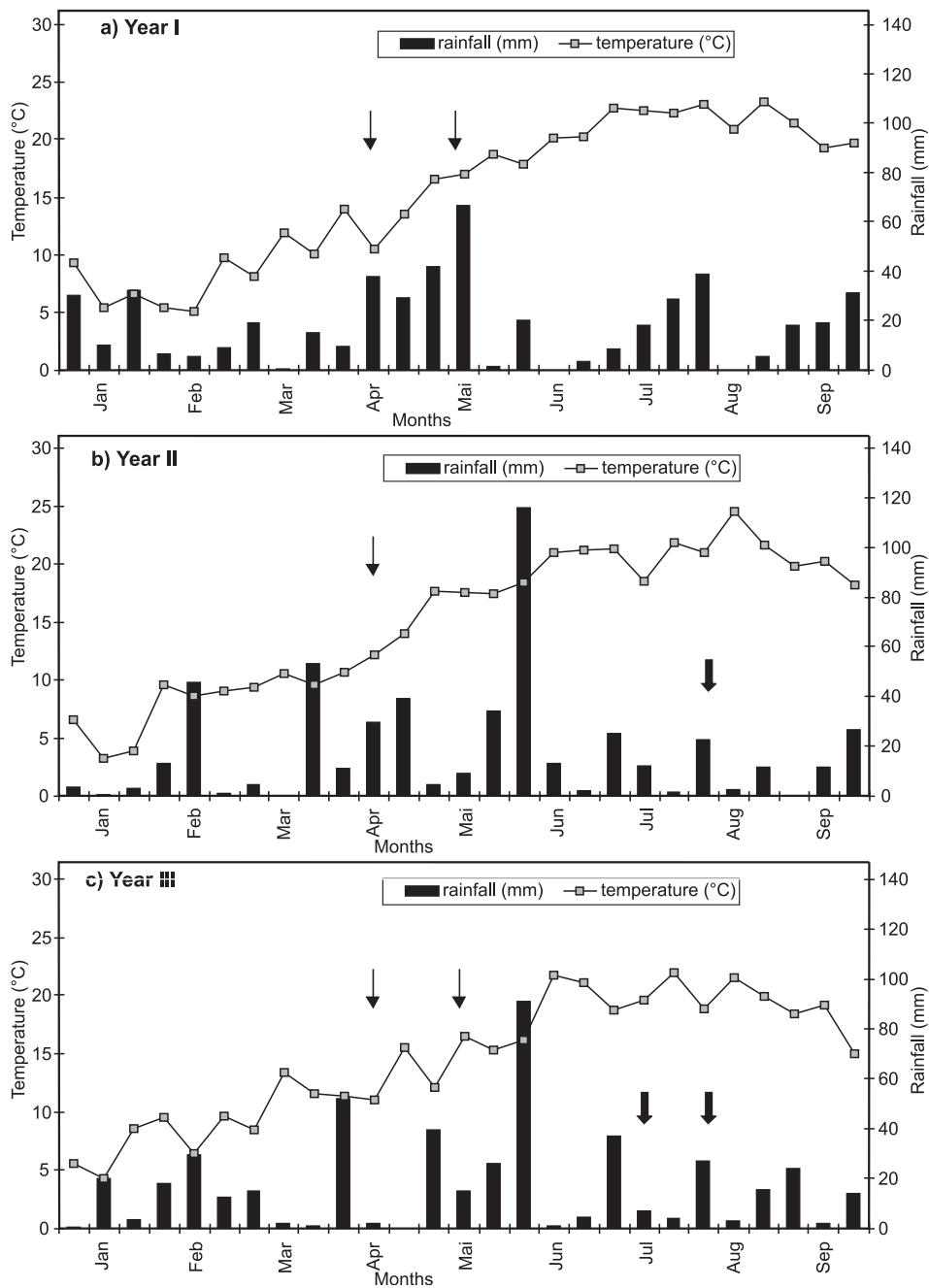
Figure 1: Rainfall and temperature mean values in: a) year I (1999), b) year II (2000) and c) year III (2002). Sowing dates are indicated by a thin arrow ( \downarrow ). The amount of irrigation applied in post-flowering period are indicated by a full arrow ( \Downarrow ).
