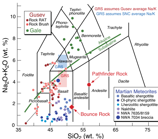
FIGURE 2. Geochemical classification of martian igneous rocks in Gusev and Gale craters analyzed by rovers ( \text{SO}_3 - and Cl-free), and of martian meteorites. Bounce Rock is a Meridiani igneous sample similar in composition to shergottites; the Mars Pathfinder rock composition is likely to be an altered surface coating. Global average GRS data (colored boxes) are consistent with basaltic compositions; GRS cannot determine Na contents, so two assumptions are made for Na/K. Updated from McSween et al. (2009).
