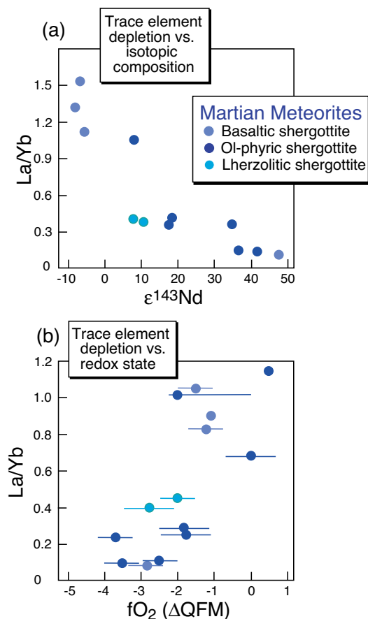
FIGURE 7. Geochemical correlations among shergottites, arising from geochemically depleted and enriched source regions. (a) Bulk ratios of light (La) to heavy (Yb) rare earth elements (normalized to chondrite) correlate with (a) radiogenic isotope compositions such as \epsilon^{143}\text{Nd} , and (b) oxidation state as measured by Fe-Ti oxide oxybarometry. Modified from McSween and McLennan (2013).
