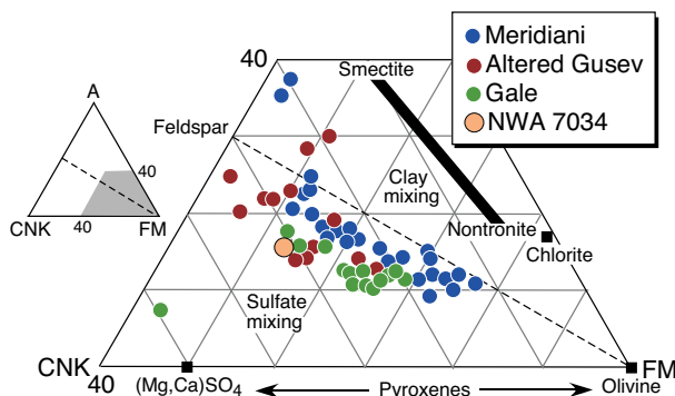
FIGURE 9. A-CN-K-FM diagram showing compositions of martian sedimentary and altered rocks. Modified from McGlynn et al. (2012), with additional analyses of Meridiani rocks (Arvidson et al. 2014), Gale crater rocks (McLennan et al. 2014), and the NWA 7034 regolith breccia (Agee et al. 2013).
