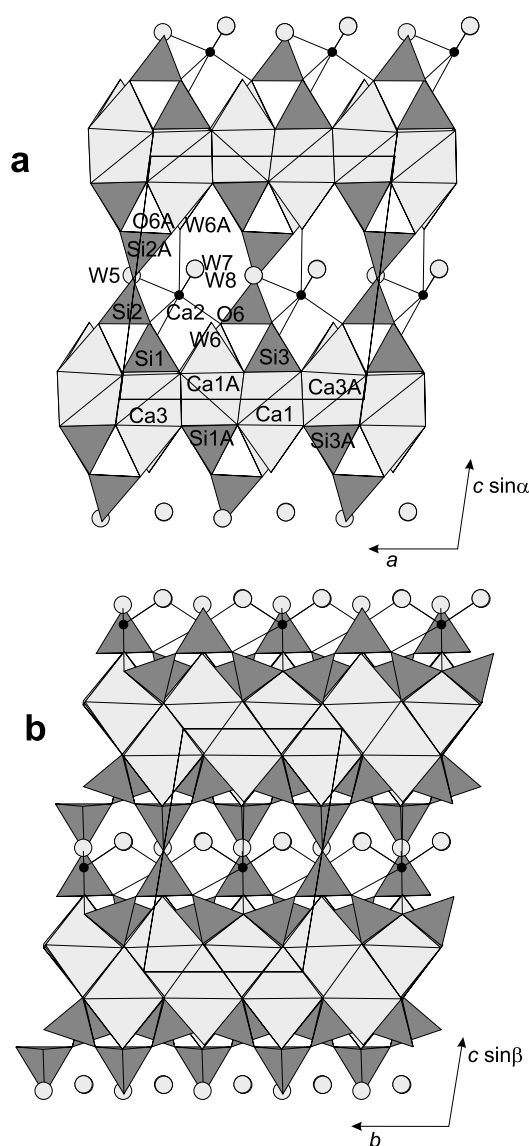
FIGURE 3. Crystal structure of the triclinic polytype \text{MDO}_2 of clinotobermorite, as seen along [010] (a) and down [100] (b). The “framework” is built up by chains of silicon tetrahedra (dark gray) and layers of sevenfold-coordinated calcium polyhedra (light gray). The calcium cation \text{Ca2} is tightly bonded to two oxygen atoms of the framework and to the “zeolitic” water molecules W5, W7 and W8.
