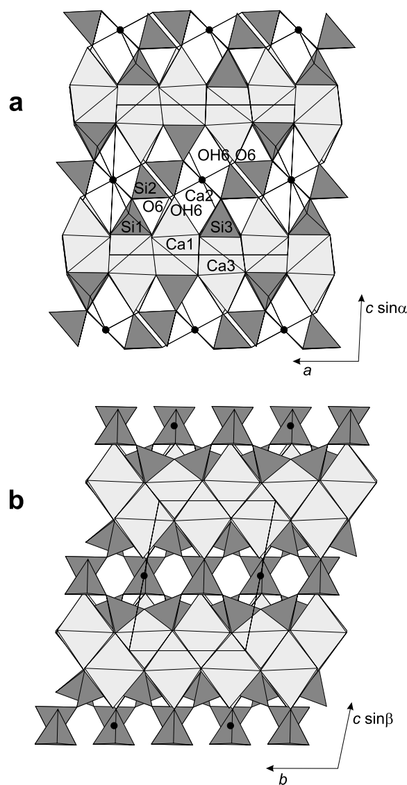
FIGURE 4. Crystal structure of the triclinic polytype \text{MDO}_2 of tobermorite 9 Å, as seen down [010] (a) and along [100] (b). The calcium cation \text{Ca2} is tightly bonded to oxygen atoms of the framework. Symbols are as in Figure 3.
