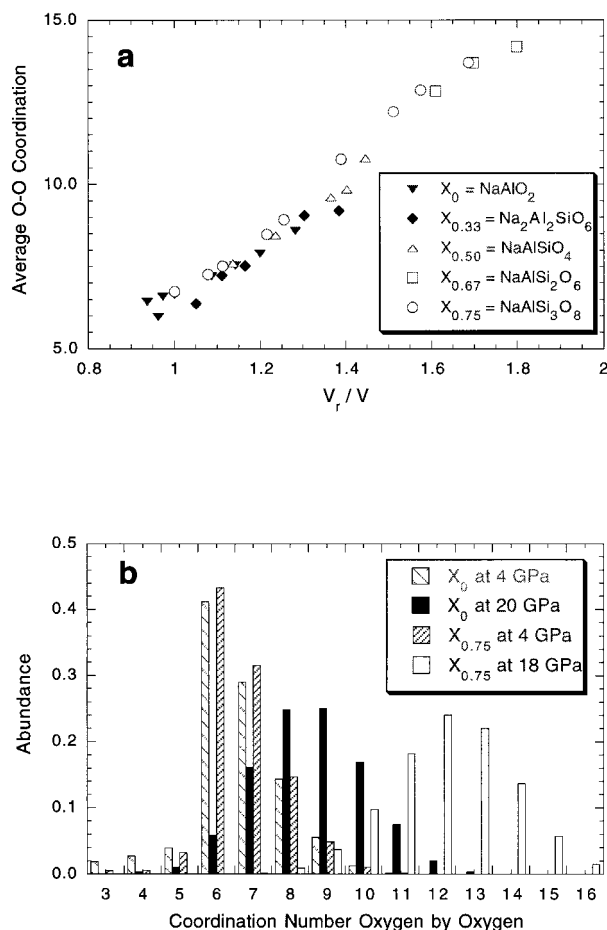
FIGURE 3. O by O coordination. (a). Average coordination of O around other O atoms plotted against compression. Symbols as in Figure 1. A somewhat steeper trend sets in at a compression of circa 1.4. This corresponds to a pressure of about 20 to 25 GPa. (b). Comparison of O by O coordination in the end-member compositions NaAlO 2 and NaAlSi 3 O 8 . The modes of O coordination at 4 GPa are similar—peaks at 6 and 7 for both molten sodium aluminate and molten albite. At higher pressures, albite tends toward higher coordination states of O and approaches face-centered cubic closest packing of O with an O by O coordination number (CN) of twelve.
