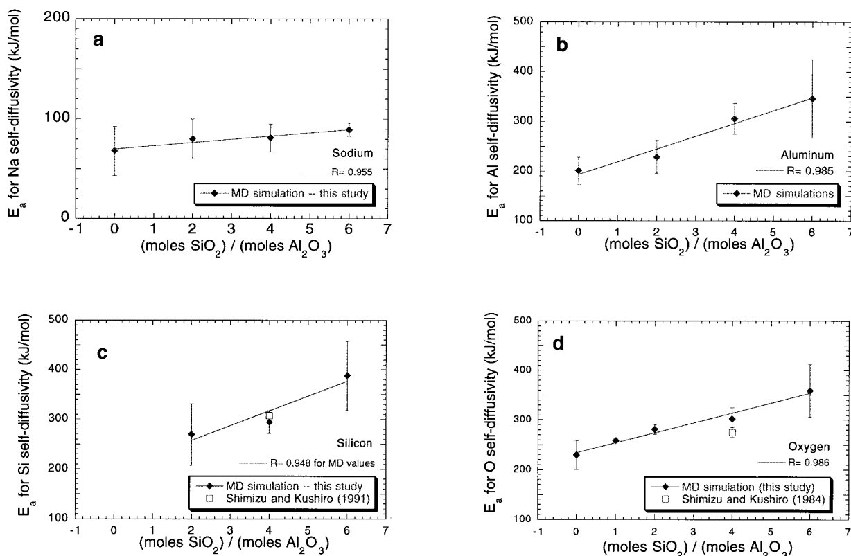
FIGURE 7. Activation energies calculated for each composition by species. (a) Trend in activation energy for Na self-diffusion compromised given the uncertainties for E_a . (b) Aluminum activation energy increases with increasing silica content of the melt. (c) Silicon activation energy behaves similarly; laboratory result of Shimizu and Kushiro (1991) plotted for comparison. (d) Activation energy for O self-diffusion also increases with increasing silica content. Laboratory results of Shimizu and Kushiro (1984) plotted for comparison (see also Bryce et al., 1997).
