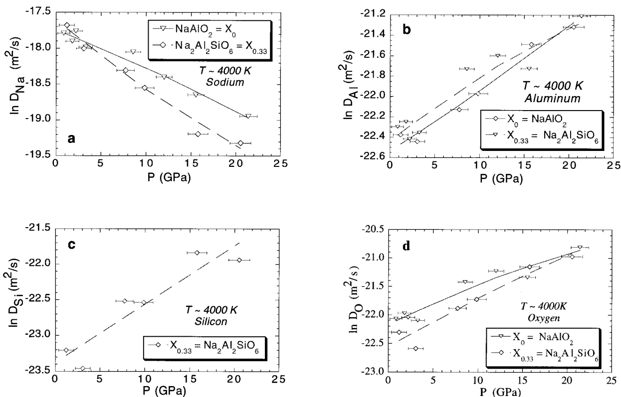
FIGURE 4. Self-diffusivity of Na (a), Al (b), Si (c), and O (d) in NaAlO 2 and Na 2 Al 2 SiO 6 melts for T \sim 4000 K as a function of pressure. Si, Al, and O all exhibit negative activation volumes, whereas Na shows a positive value. Typical reproducibility in \ln D values range from <0.2 (ln D units) for Na to <0.4 (ln D units) for O, Si, and Al.
