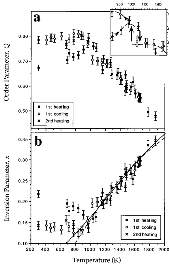
FIGURE 2. Temperature dependence of (a) the order parameter ( Q ) and (b) inversion parameter ( x ), for cation order-disorder in spinel, from in situ neutron diffraction. Circle = data obtained at IPNS; X = data obtained from the same sample during a subsequent in situ heating experiment at ISIS. The dashed line in b is a fit to the equilibrium data between 560 and 1600 °C using the O'Neill and Navrotsky (1983) thermodynamic model (Eq. 3), yielding \alpha = +32.8 \pm 0.9 kJ/mol and \beta = +4.7 \pm 2.0 kJ/mol. The solid line shows the fit to the Landau expression for ordering (Eq. 6) with values of T_c = 445 \pm 109 K and c' = 1.62 \pm 0.21 .
