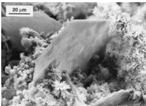
FIGURE 1. SEM photograph of a thin, tabular gordaite crystal of hexagonal habit, associated with tiny barite aggregates from the Juan de Fuca Ridge, northeastern Pacific Ocean.
